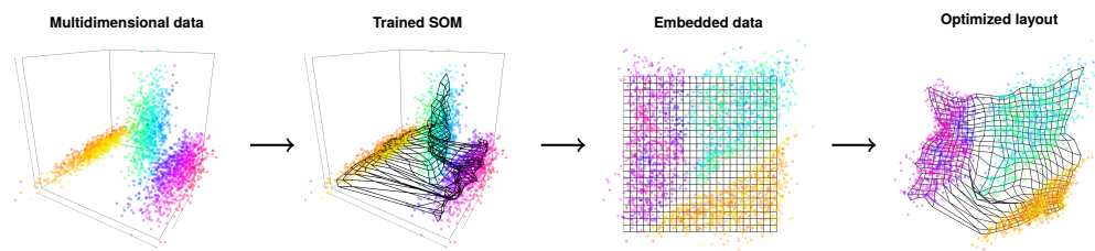
Figure 4: Overview of the EmbedSOM embedding process, shown on three synthetic Gaussian clusters in 3-dimensional space. From left: The cells in multi-dimensional space are used to train a SOM that describes their distribution; embedding then smoothly fits the content of multi-dimensional space to a flat version of SOM. Finally, result can be quickly optimized by changing embedding parameters and SOM layout (in the picture, the lengths of grid edges are optimized to match values in the corresponding U-matrix), and efficiently recomputing only the last algorithm stage.
