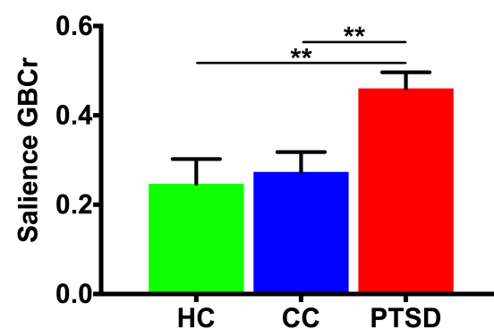
Figure 3. Overall Salience Global Connectivity in US Army Soldiers with Posttraumatic Stress Disorder (PTSD). There was a significant main group effect with increased overall (i.e., at rest and during trauma recollection) global brain connectivity with global signal regression (GBCr) in PTSD compared to combat (CC) and healthy controls (HC). ** P \leq .01 .
