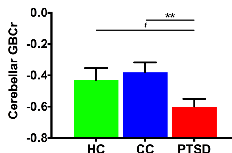
Figure S1. Overall Cerebellar Global Connectivity in US Army Soldiers with Posttraumatic Stress Disorder (PTSD). There was a significant main group effect with increased overall (i.e., at rest and during trauma recollection) global brain connectivity with global signal regression (GBCr) in PTSD compared to combat controls (CC), with a trend level significance, compared to healthy control (HC). ** P \leq .01 ; * P \leq .1 .
