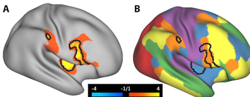
Figure 1. Cortical Global Connectivity in US Army Soldiers with Posttraumatic Stress Disorder (PTSD). A. The orange-yellow clusters mark the vertices with increased global brain connectivity with global signal regression (GBCr) in PTSD compared to controls during symptom provocation. The black lines mark the vertices with P < .005 and corrected \alpha = .05 . B. The map of 6 intrinsic connectivity networks: ventral salience (blue), dorsal salience (orange), central executive (yellow), default mode (green), visual (red), and sensorimotor (purple). The black lines in B mirror the black lines in A.
