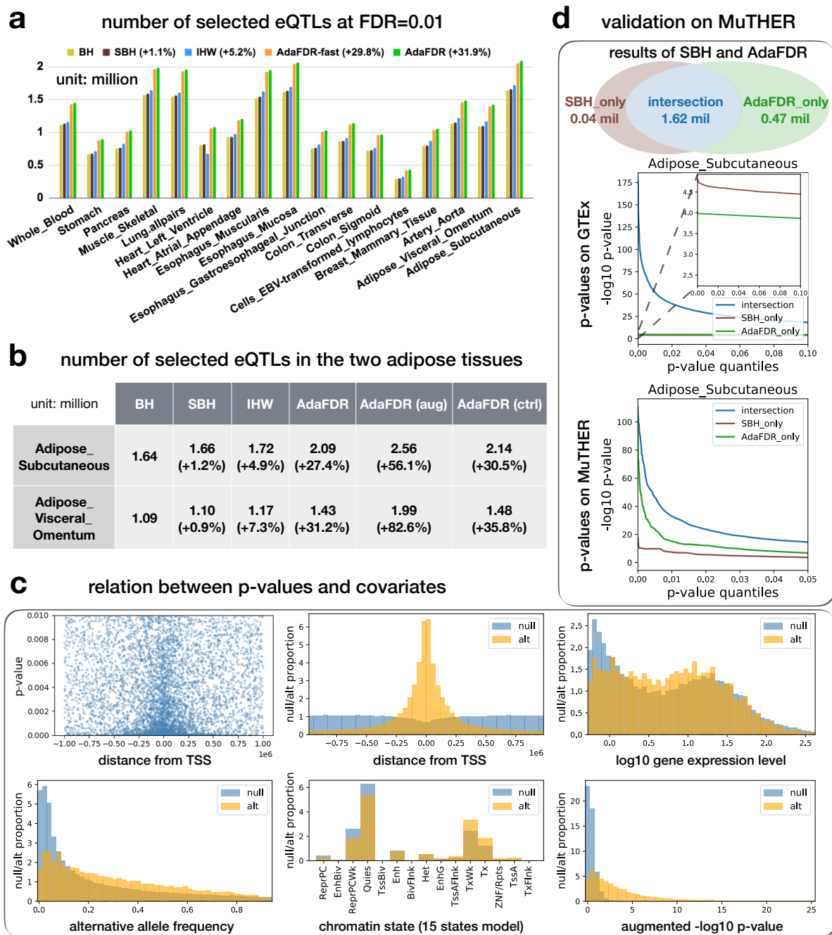
Figure 2. Analysis of the GTEx data. (a) Results of 17 tissues considered in the study. AdaFDR and its fast version consistently make more discoveries than other methods. (b) Results on the two adipose tissues where the -\log_{10} p-value from another tissue was added as an extra covariate. Using p-values from a similar tissue (AdaFDR (aug)) yields significantly more discoveries than using p-values from an unrelated tissue (AdaFDR (ctrl)). (c) Top-left: P-values (y-axis) plotted against the distances from TSS (x-axis); each dot corresponds to one SNP-gene pair. Small p-values at the center suggest that hypotheses with smaller distances from TSS are more likely to be significant. Other panels: AdaFDR-estimated null hypothesis distribution (blue) and alternative hypothesis distribution (orange) with respect to each covariate. Higher values of the orange distribution suggest an enrichment of alternative hypotheses. (d) Top: Discoveries made by SBH and AdaFDR. Middle: The p-values of these discoveries—SBH-only p-values are smaller than AdaFDR-only p-values on GTEx. Bottom: The p-values of the same set of discoveries on the independent MuTHER data, where AdaFDR-only p-values are smaller than SBH-only p-values, suggesting that AdaFDR-only discoveries are more likely to be true discoveries.
