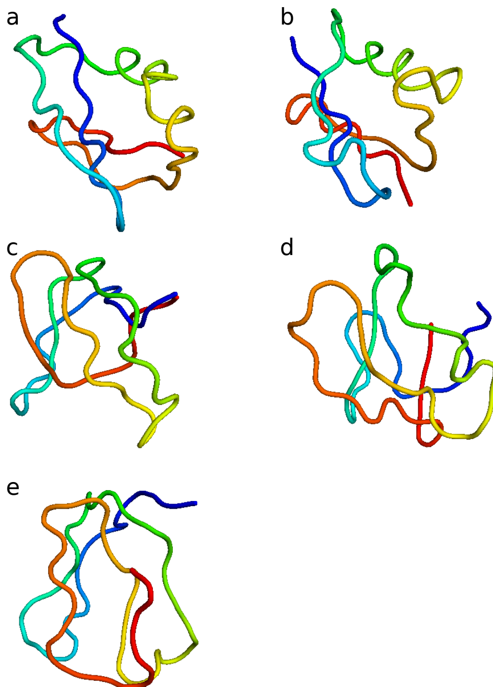
Figure S3: Reconstruction of protein structures from simulated contact frequency data. Shown is the MAP estimate for n = 5 states.
