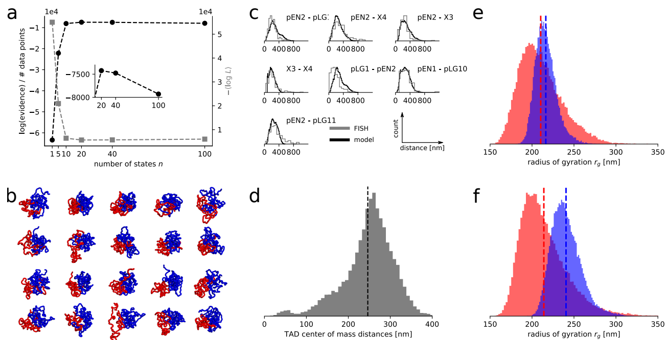
Figure 3: Inference of multi-state chromatin models from 5C data on male (a–d) and female (e, f) mESCs.
