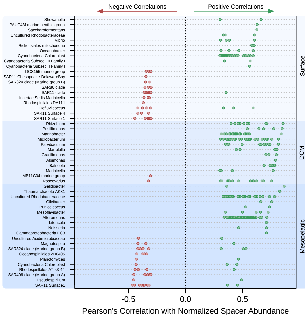
Fig. 2. CRISPR abundance correlates with several taxonomic OTU's, with stronger positive correlations in deeper ocean zones. The top 10 positively and negatively correlating OTUs with respect to normalized spacer abundance, broken down by oceanic depth zone. Some taxa have several significant OTUs.
