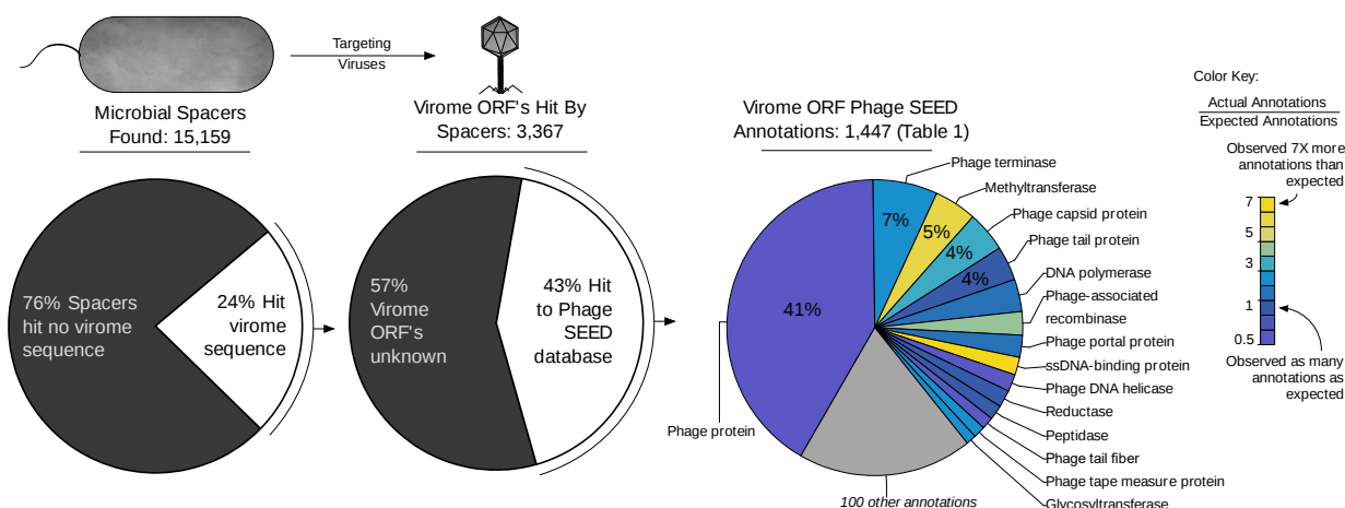
Fig. 4. Microbial spacers preferentially target specific viral genes. Nearly one quarter of aquatic microbial spacers had a putative match to aquatic virome genes. The majority of these genes obtained informative annotations (i.e. not “Phage protein”). Most genes targeted by CRISPR spacers were annotated two-fold as often as expected, based on the expected frequencies of aquatic virome gene annotations. Two gene annotations that were seen less frequently than expected were DNA helicase and phage tail fiber.
