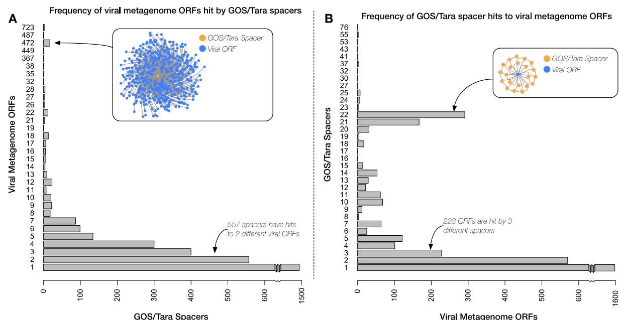
Fig. 3. CRISPR spacers aligned with viral gene targets in a many-to-many relationship. (A) Frequency of viral metagenome ORFs hit by GOS and Tara Oceans spacers with inset network graph representing the 1 to 472 relationship. (B) Frequency of GOS and Tara Oceans spacer hits to viral metagenome ORFs with inset network graph representing the 22 to 1 relationship.
