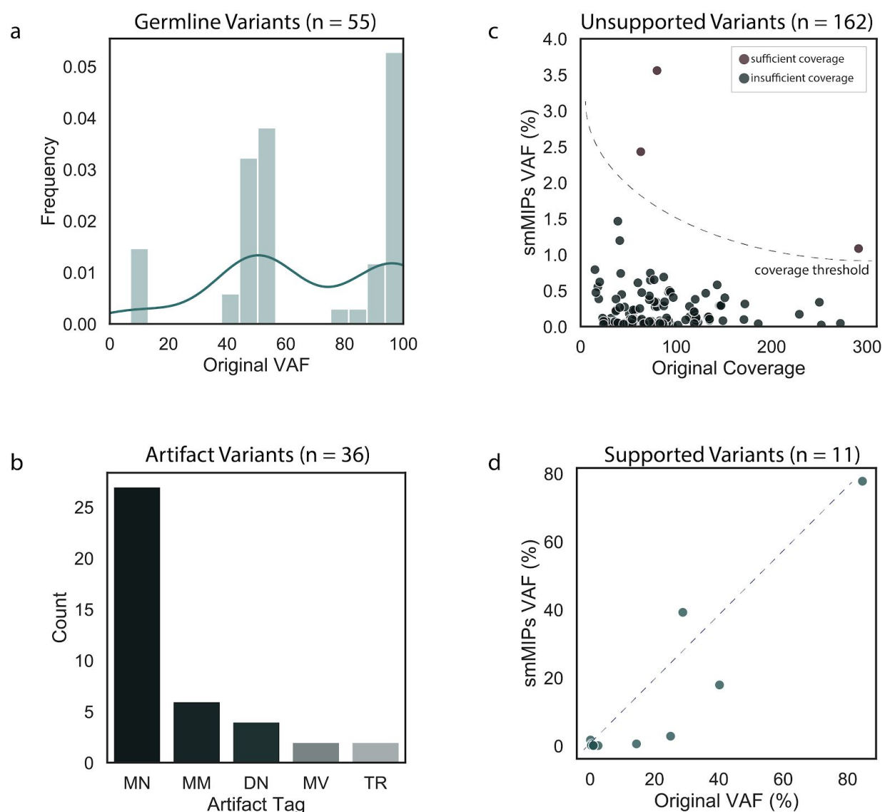
Figure 5. Analysis of variants rescued by CIViC smMIPs sequencing for samples with both tumor and matched normal. There were 217 variants called as somatic by the CIViC smMIPs sequencing that were not identified on original sequencing. All variants were manually reviewed using both CIViC smMIPs sequencing data and original sequencing data a. During manual review 55 variants were identified as germline. A histogram shows that the distribution of the smMIPs VAF for these germline variants are observed at 50% and 100% VAF, indicating heterozygosity and homozygosity, respectively. b. An additional 36 variants were identified as sequencing artifacts. Most artifacts were either mononucleotide repeats (MN), dinucleotide repeats (DN), or tandem repeats (TR). Other artifacts include multiple mismatches (MM) or multiple variants (MV). c. During manual review, 162 variants did not show any support in the original sequencing data. Most unsupported variants did not have sufficient coverage to be detected based on a binomial probability of at least 4 variant-supporting reads (see Methods ). d. The remaining 11 variants had variant support in original sequencing but were not called as somatic in final original annotation. Scatter plot shows correlation between original VAF and CIViC smMIPs VAF for these variants.
