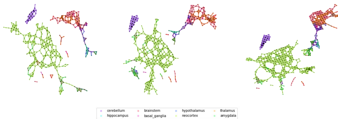
Figure 5: (Colour online) Mapper networks on reduced Richiardi functional list. From left to right, we show some Mapper networks obtained for different overlaps between bins (overlap 0.25, 0.3, 0.35). The networks displays the separation of the cerebellum and two larger components, composed by cortical and subcortical areas respectively, which we further characterize using the agreement matrices.
