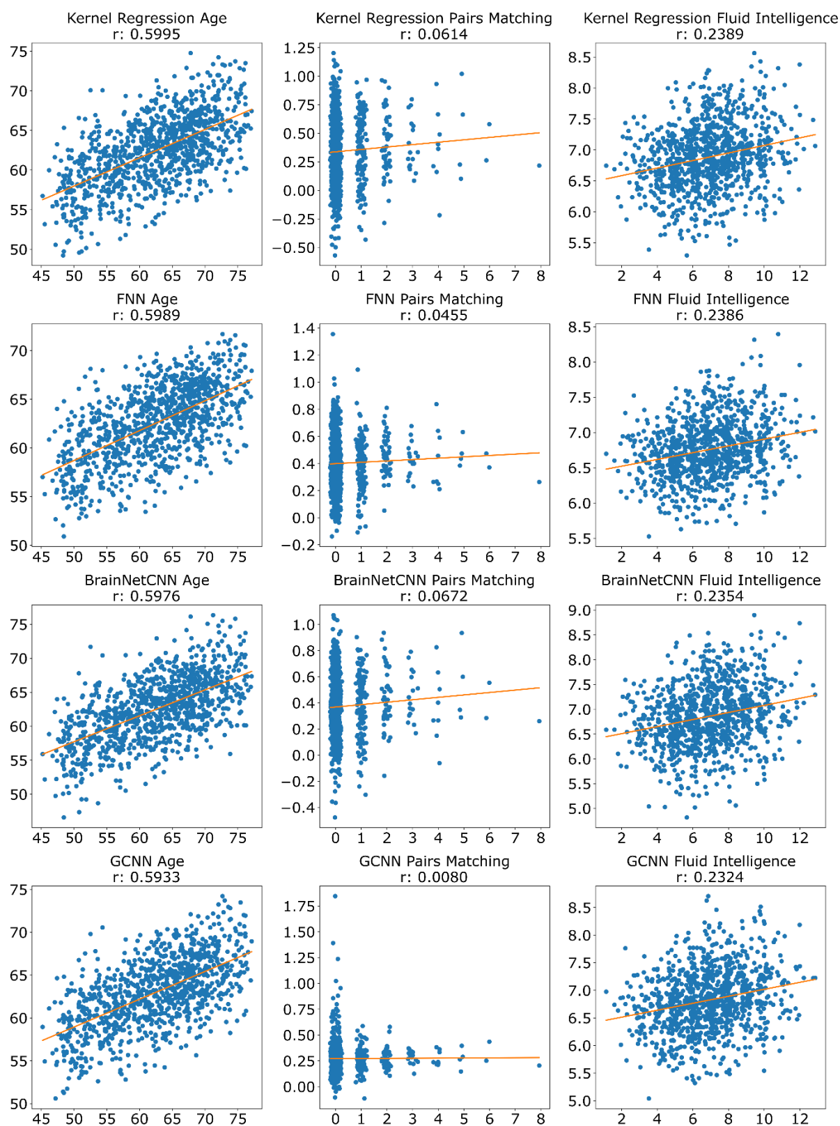
Figure S9. Scatterplots of predicted versus actual values for age, pairs matching and fluid intelligence for the 1000 UK Biobank subjects in the test set. X-axis is the actual value. Y-axis is the predicted value. Each dot represents one subject. The orange line shows the best fit line obtained by least squares regression. The “r” in each subplot title is the Pearson’s correlation coefficient between the predicted and actual values, which was also reported in Table 1.
