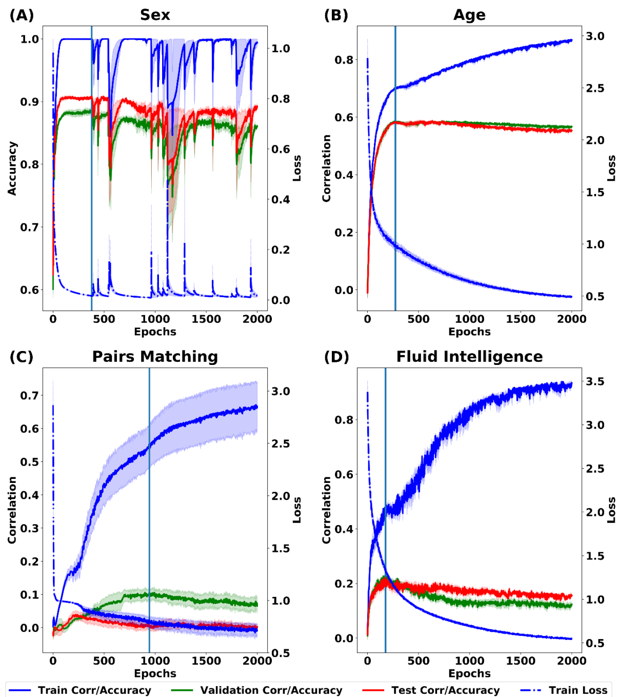
Figure S15. Learning curves of GCNN for the UK Biobank using the final set of hyperparameters. Blue solid curve shows the training correlation (or accuracy for sex prediction). Blue dot curve shows the training loss. The green curve shows the validation correlation (or accuracy for sex prediction). The red curve shows the testing correlation (or accuracy for sex prediction). The shadow represents the standard error across the five ensemble runs. The blue vertical line indicates the stopping point, which corresponded to the best validation correlation/accuracy.
