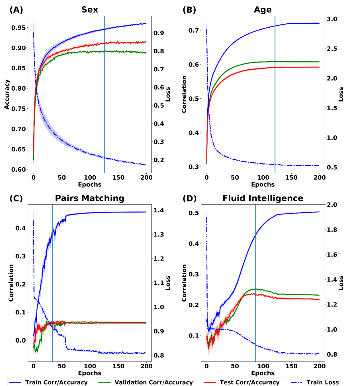
Figure S14. Learning curves of BrainNetCNN for the UK Biobank using the final set of hyperparameters. Blue solid curve shows the training correlation (or accuracy for sex prediction). Blue dot curve shows the training loss. The green curve shows the validation correlation (or accuracy for sex prediction). The red curve shows the testing correlation (or accuracy for sex prediction). The shadow represents the standard error across the five ensemble runs. The blue vertical line indicates the stopping point, which corresponded to the best validation correlation/accuracy.
