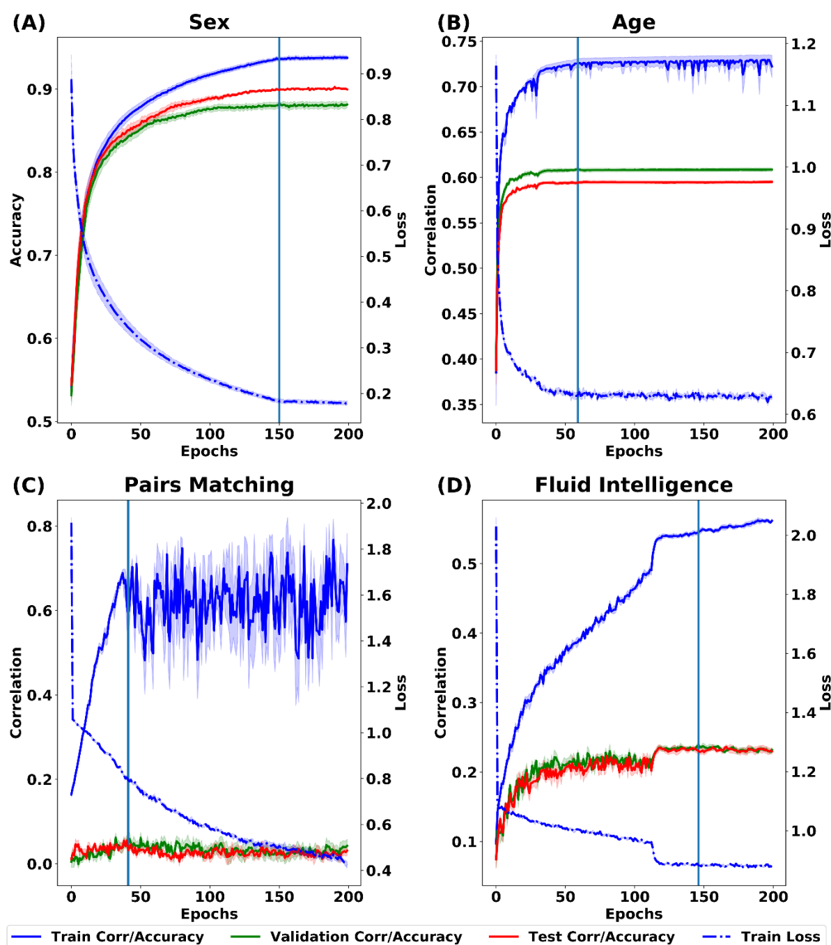
Figure S13. Learning curves of FNN for the UK Biobank using the final set of hyperparameters. Blue solid curve shows the training correlation (or accuracy for sex prediction). Blue dot curve shows the training loss. The green curve shows the validation correlation (or accuracy for sex prediction). The red curve shows the testing correlation (or accuracy for sex prediction). The shadow represents the standard error across the five
