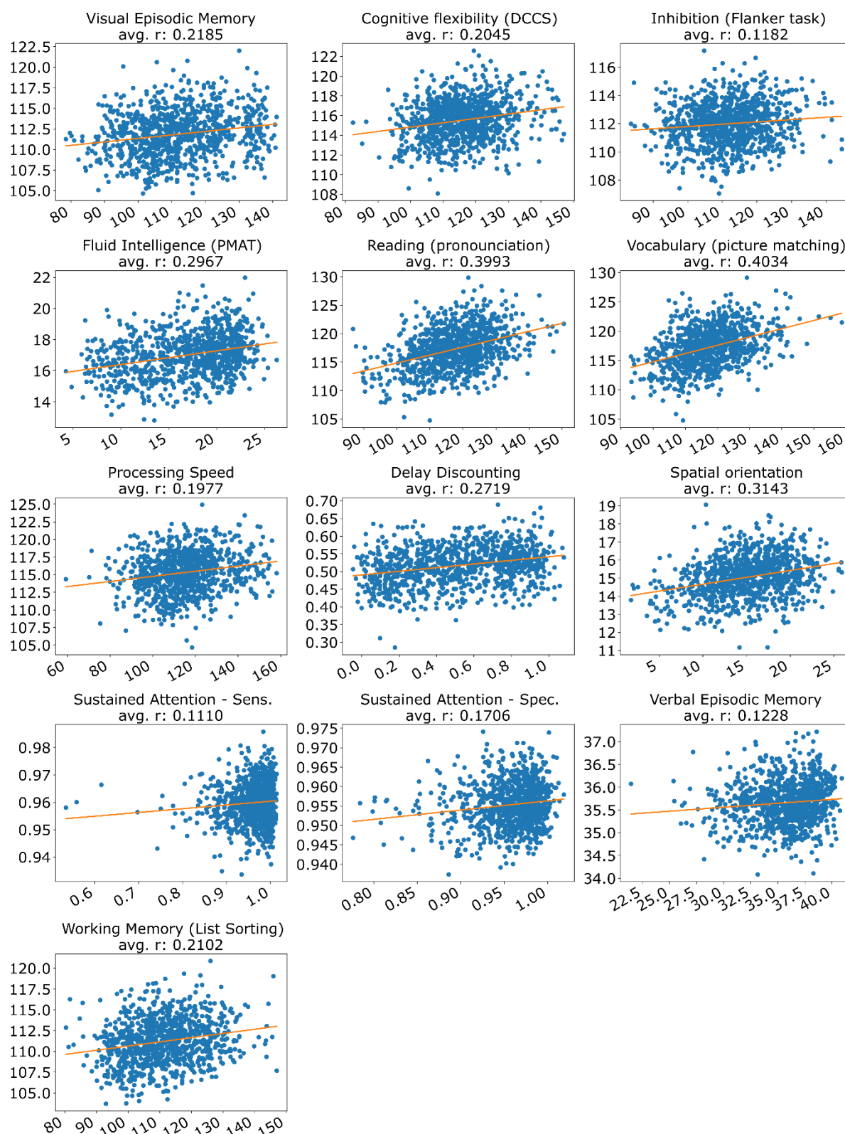
Figure S5. Scatterplots of predicted (FNN) versus actual values for a curated set of 13 HCP cognitive measures for all 953 subjects. X-axis is the actual value. Y-axis is the predicted value. Each dot represents one subject. The orange line shows the best fit line obtained by least squares regression. The “avg. r” in each subplot title is the average Pearson’s correlation coefficient across 20 test folds, which was also reported in Figure 5.
