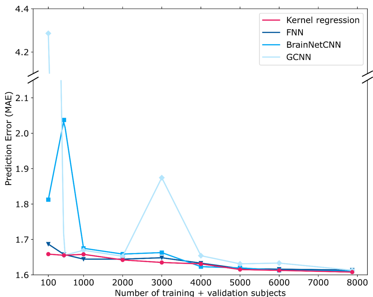
Figure S11. Prediction error (MAE) of fluid intelligence in the UK Biobank dataset with different number of training and validation subjects. Lower MAE represents better performance. The performance of all algorithms generally improved as the number of training and validation subjects increased. In the case of 100, 500, 1000 and 2000 subjects, 3/4 of the subjects were used for training and 1/4 of the subjects were used for validation. In the remaining cases, 1000 subjects were used for validation, while the remaining subjects were used for training. For all cases, test set comprised the same set of 1000 subjects. Kernel regression was highly competitive across all sample sizes.
