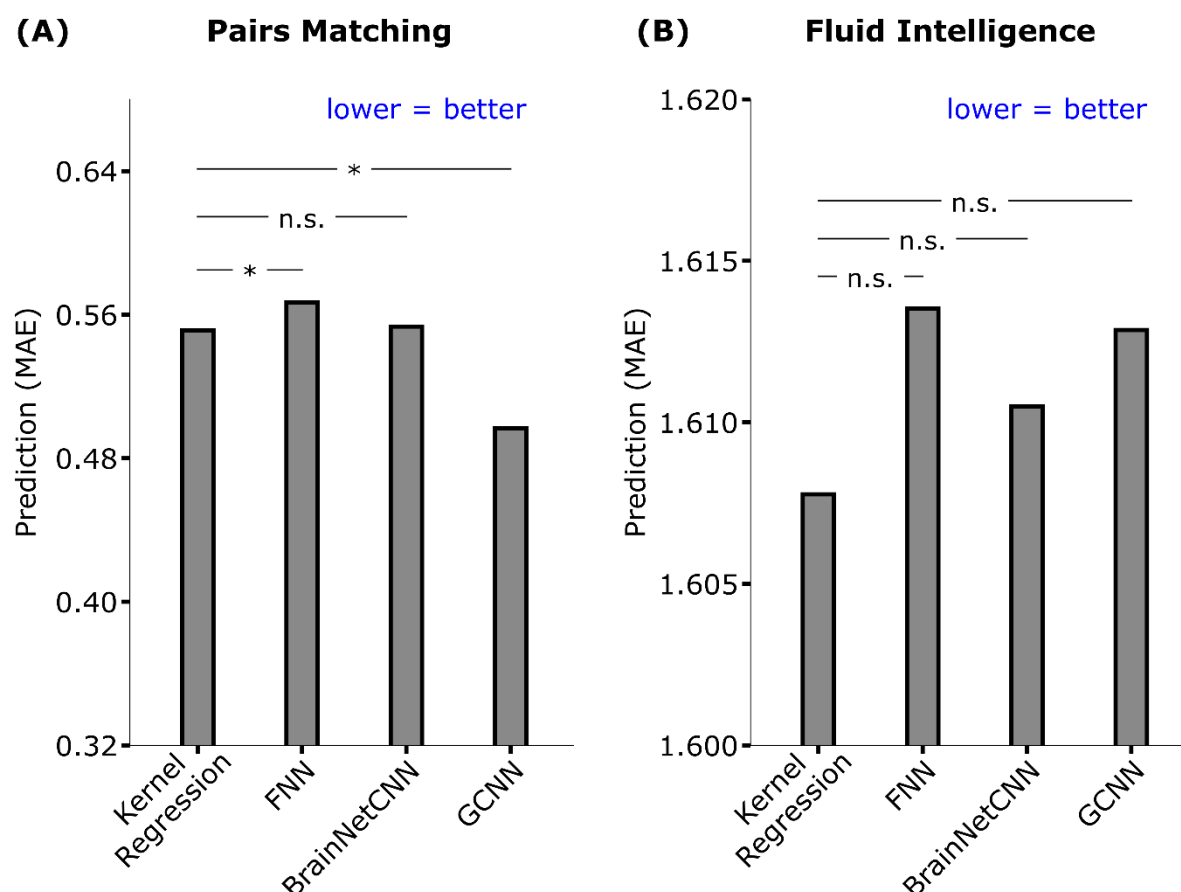
Figure S10. Prediction MAE of pairs matching and fluid intelligence in the UK Biobank. Lower values imply better performance. The horizontal lines represent statistical tests between kernel regression and the DNNs. “n.s.” stands for not significant. “*” implies statistical significance after FDR ( q < 0.05 ) correction. In the case of pairs matching, kernel regression was statistically better than GCNN ( p = 1e-10 ), but statistically worse than BrainNetCNN ( p = 0.009 ). However, we note that all algorithms performed worse than simply predicting the median pairs matching value in the training set, which would have yielded an MAE of 0.4.
