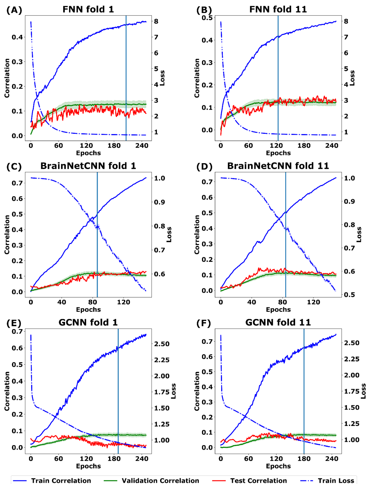
Figure S12. Learning curves of DNNs for folds 1 and 11 of the HCP dataset using the final set of hyperparameters. Blue dot curve shows the training loss averaged across 19 training curves during the inner-loop cross-validation. The green curve shows the validation correlation averaged across 58 behavioral measures and 19 validation curves during the inner-loop cross-validation. The shadow (for training loss and validation correlation) represents the standard error across 19 training and validation curves. The blue vertical line
