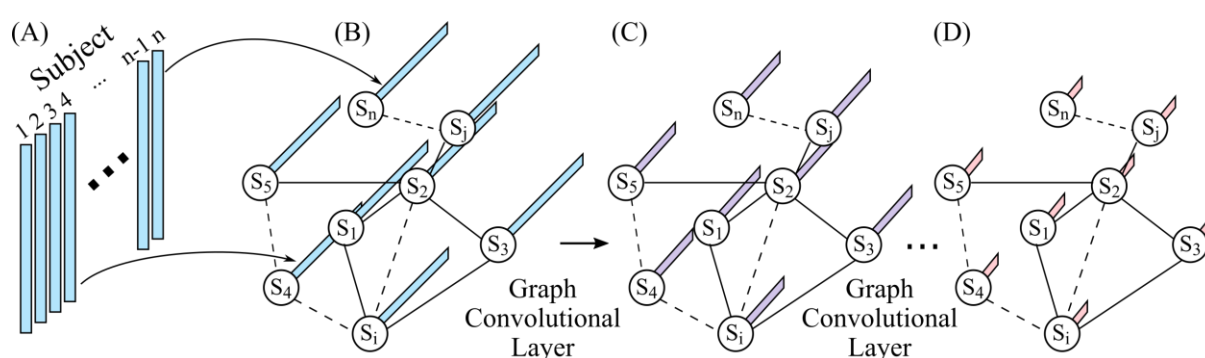
Figure 3. Schematic of a graph convolution neural network (GCNN; Parisot et al., 2017, 2018). This particular GCNN takes in vectorized RSFC matrices of all subjects as input and outputs behavioral (or demographic) prediction of all subjects. (A) Vectorized FC of all subjects (subject 1 to subject n). (B) The input of GCNN is a graph, where each node represents a subject and is associated with the vectorized FC from the corresponding subject in (A). An edge in the graph represents the similarity between two subjects. Here, the similarity is defined in terms of the similarity of the subjects' RSFC matrices. (C) Output of the first graph convolutional layer. Graph convolutional layer extends standard convolution to graph convolution. Each node is associated with a vector, whose length is determined by the number of filters in the first graph convolutional layer. (D) Final output of GCNN after one or more graph convolutional layers. Each node contains the predicted behavioral measure(s).
