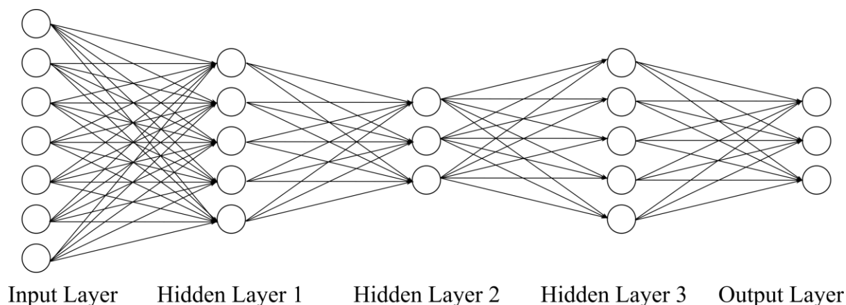
Figure 1. Schematic of a feedforward neural network (FNN). An FNN takes in vectorized RSFC matrix entries as inputs and outputs behavioral or demographic predictions. An FNN consists of an input layer, several hidden layers (three layers are shown here) and an output layer. The number of nodes in the input layer is equal to the number of elements in the lower triangular portion of the RSFC matrix. The number of nodes in the output layer is typically equal to the number of behavioral measures we are predicting. The number of hidden layers and number of nodes in the hidden layers are among the many hyperparameters that have to be tuned.
