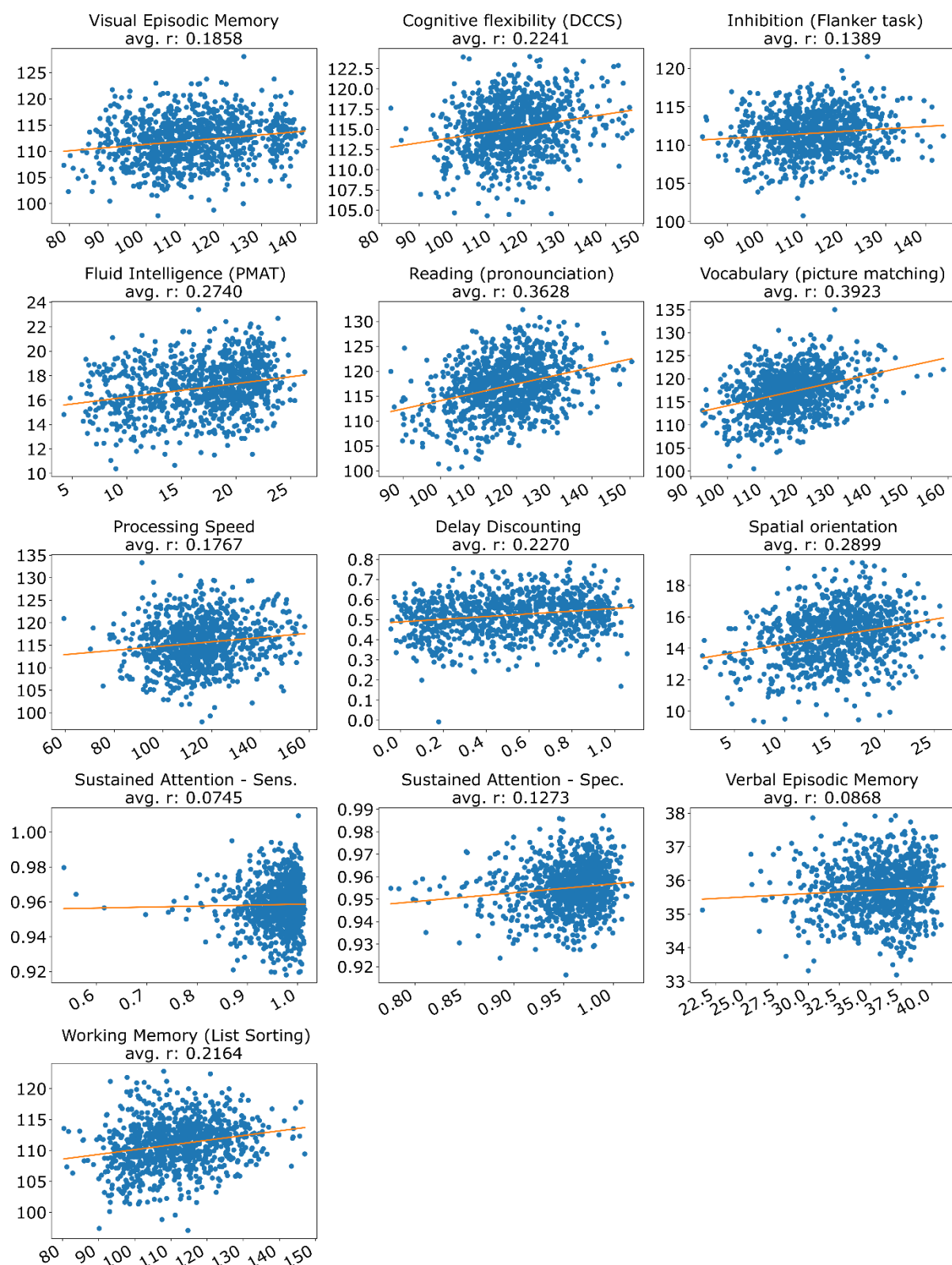
Figure S6. Scatterplots of predicted (BrainNetCNN) versus actual values for a curated set of 13 HCP cognitive measures for all 953 subjects. X-axis is the actual value. Y-axis is the predicted value. Each dot represents one subject. The orange line shows the best fit line obtained by least squares regression. The “avg. r” in each subplot title is the average Pearson’s correlation coefficient across 20 test folds, which was also reported in Figure 5.
