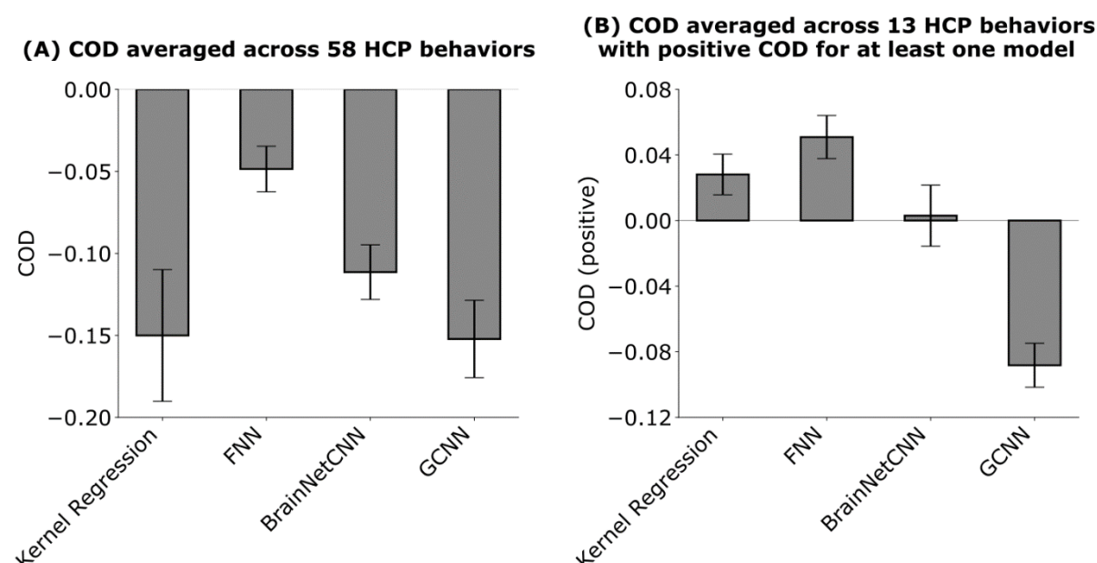
Figure S8. Prediction COD (coefficient of determination) averaged across HCP behavioral measures and 20 test folds. (A) Prediction COD averaged across all 58 behavioral measures. COD was computed for each test fold and each behavior and then averaged across the 58 behaviors and 20 test folds. Bars show the mean across test folds. Error bars show standard error of model performance across cross-validation folds. There was no statistical difference between kernel regression and all DNNs after correcting for multiple comparisons. (B) Prediction COD averaged across 13 behavioral measures. The negative COD in (A) suggests that there were a number of measures that were predicted poorly across all methods. Therefore, we considered a subset of measures with positive COD for at least one regression model (kernel regression, FNN, BrainNetCNN and GCNN). There were 13 such measures, so we averaged the COD across the 13 measures. Bars show the mean across test folds. Error bars show standard error of model performance across test folds.
