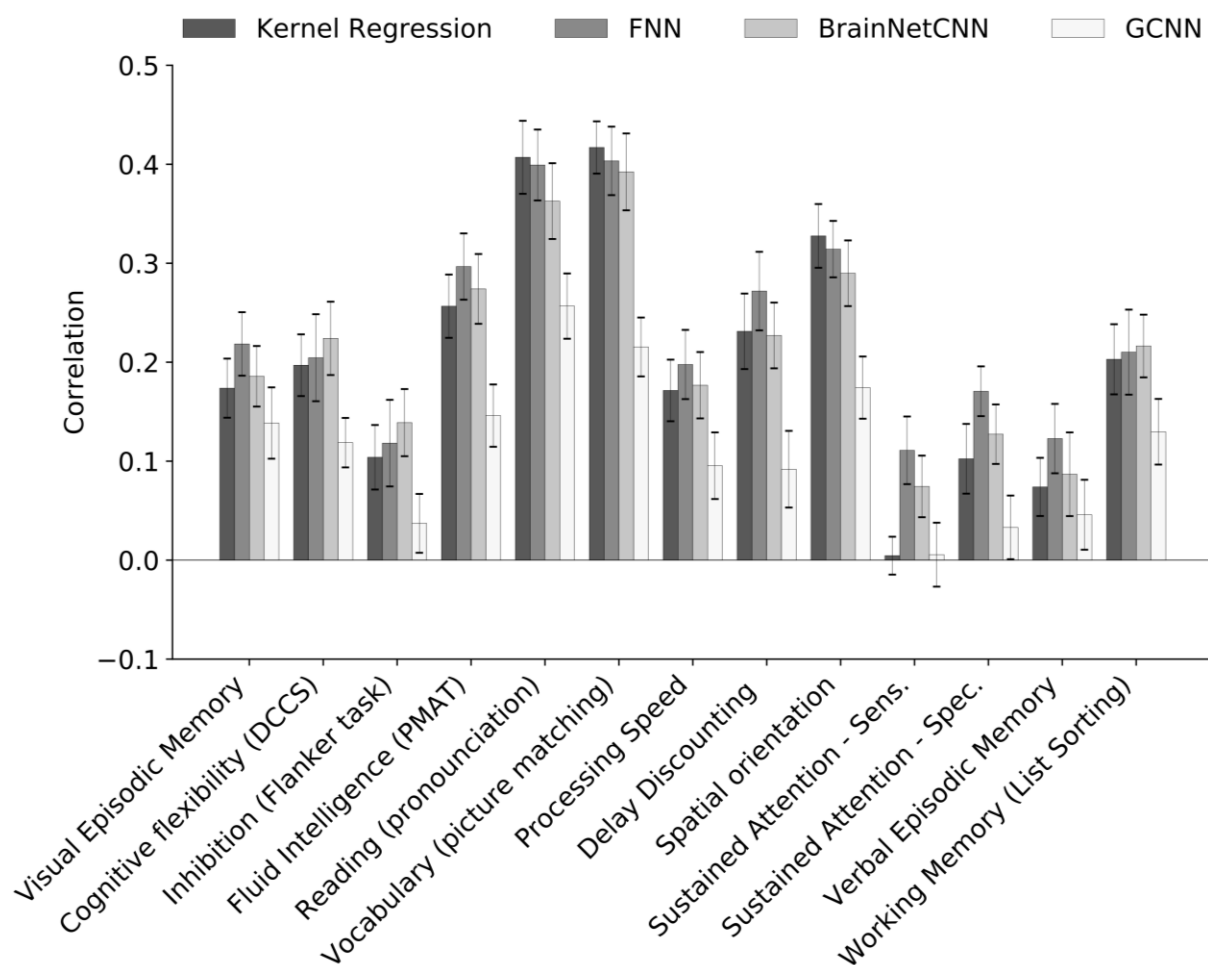
Figure 5. Prediction accuracies (Pearson's correlation coefficient) in a curated set of 13 HCP cognitive measures averaged across 20 test folds. Correlation was computed for each test fold and each behavior. Bars show mean across test folds. Error bars show standard errors of model performance across cross-validation folds. Prediction accuracies of the remaining 45 behavioral measures are found in Figures S2 and S3.
