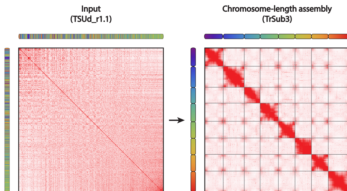
Figure 1: Hi-C map of the draft and chromosome-length assemblies of Trifolium subterraneum genome. Contact matrices were generated by aligning the same Hi-C data set to TSUd_r1.1 draft genome (left) and the TrSub3 genome assembly generated using Hi-C (right). Pixel intensity in the matrix indicates how often a pair of loci collocate in the nucleus. The correspondence between loci in the draft and final assemblies is illustrated using chromograms. The chromosome-scale assembly scaffolds in TrSub3 are assigned a linear color gradient, and the same colors are then used for the corresponding loci in the TSUd_r1.1 (left). The draft scaffolds are ordered by sequence name. Grid lines highlight the boundaries of eight chromosome-length scaffolds in TrSub3 (right). Scaffolds smaller than 10kb in TSUd_r1.1 are not included in this illustration.
