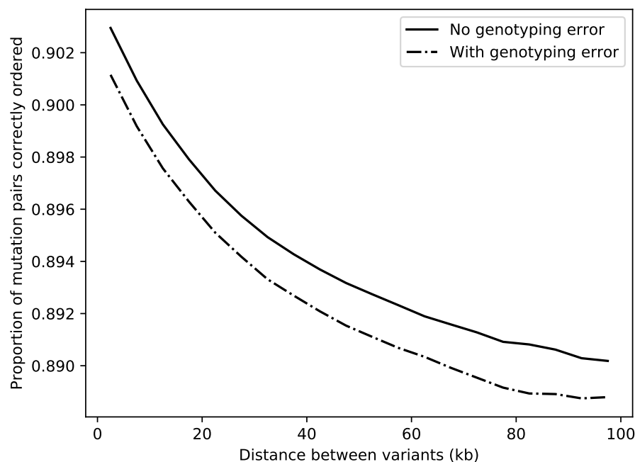
Figure S1: Accuracy of frequency as a proxy for relative age. 50 sample sequences of 100kb were simulated using msprime with N_e = 5000 and \mu = \rho = 10^{-8} . For all pairs of variant sites, the difference in mutational age was compared to the difference in frequency between the two derived alleles. If T(a_1) and T(a_2) are the ages of the derived alleles at sites 1 and 2 respectively, and f(a_1) and f(a_2) are their current frequencies in the population, frequency is said to correctly predict age order if T(a_1) < T(a_2) \implies f(a_1) < f(a_2) . We show the proportion of pairs for which frequency provides the correct order of mutation age. Results were binned into 5kb intervals and averaged over 250,000 replicates. Correlation of adjacent tree topologies results in frequency being a better predictor of relative age when variants are physically close to one another. Note that singletons have been included when calculating the statistics in this figure; removing singletons (which are not used for tsinfer inference) results in an average accuracy roughly 5% lower than shown here.
