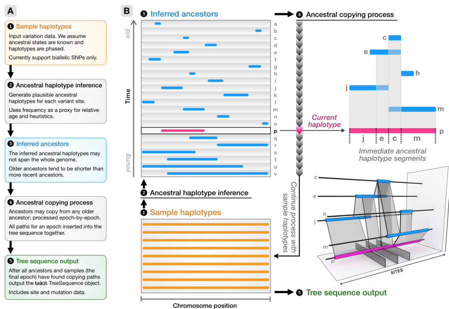
Figure 2: A schematic of the major steps of the inference algorithm. Starting from a set of sample haplotypes extending over the genome (1), we use the ancestral haplotype inference method (2) to reconstruct fragments of ancestral sequence (3), then infer copying paths among these ancestors (4). The ancestral copying process is shown on the right, using an arbitrary haplotype ( p ) for illustration. As we move from left to right along p we infer that it has most recently copied from j , e , c and then m . Incorporating the copying history of all older haplotypes (for example, m copied partly from c and partly from h ), partial coalescent trees emerge in the bottom-right panel. Once copying paths have been found for all ancestors and samples, we output a tskit tree sequence (5).
