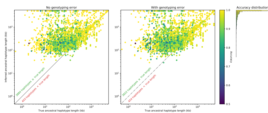
Figure S3: Accuracy of inferred ancestral haplotypes. True ancestral haplotypes were obtained from a single simulation of 100 sample sequences, each of 5Mb in length, using msprime with N_e = 5000 , and \mu = \rho = 10^{-8} . A typical result is shown here, with all \sim 4300 separate ancestral haplotypes plotted as individual points. Accuracy measures the fraction of correctly reconstructed sites, the calculation being restricted to the region in which the true and reconstructed haplotypes overlap.
