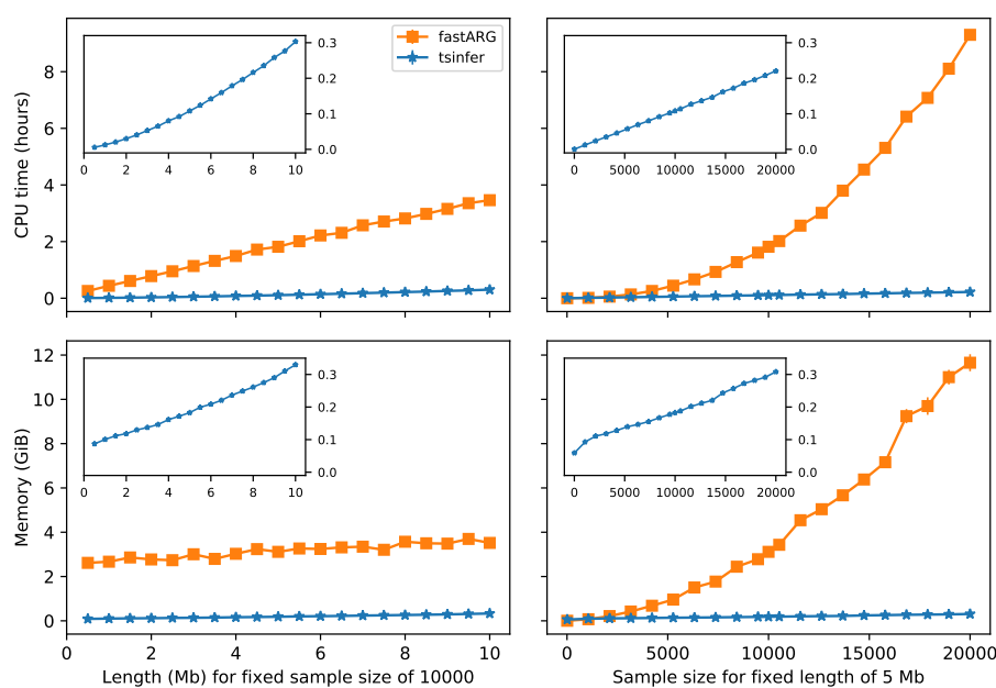
Figure S10: CPU time and memory requirements for tsinfer and fastARG , as a function of sample size and sequence length. Sequences were simulated using msprime , setting N_e = 5000 and \mu = \rho = 1 \times 10^{-8} , then used for inference without imposing genotyping error. Each point represents an average over 50 replicates. The scaling properties of tsinfer are hard to examine using the same y-axis scale as for fastARG , hence the inset plots show the tsinfer line only, with a rescaled y-axis.
