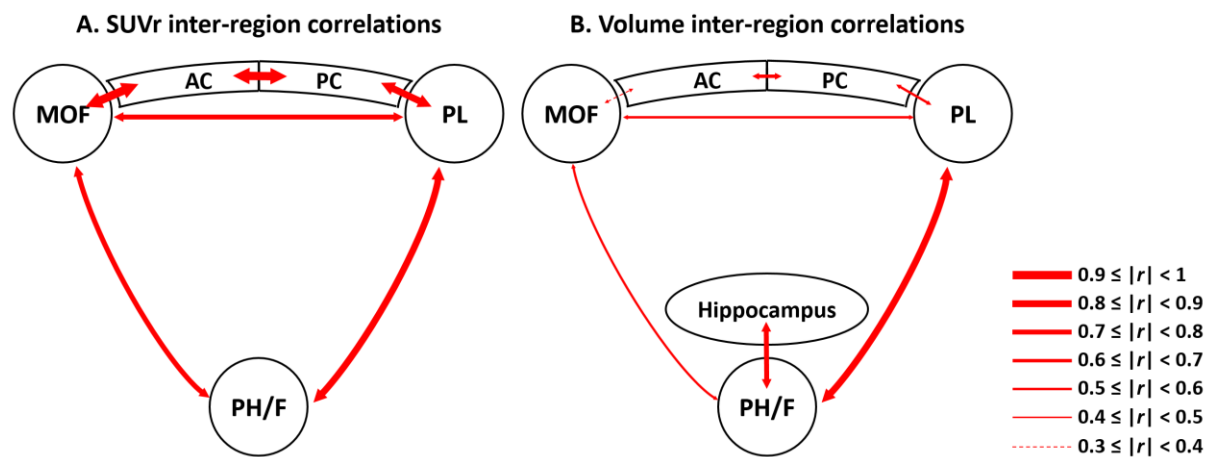
Figure 2. Significant correlations between SUVR's (A) or volumes (B) of cortical regions directly connected by WM tracts. The thickness of the red arrows illustrates the strength of the correlation. All correlation values are provided in Tables 1 and 2.
