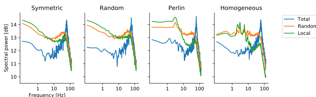
Figure 4: Power spectra of network activity in different spatial inhomogeneity configurations in I-networks. Power spectra of summed spiking activities (bin width = 4ms), with different traces referring to the source of the data: the z-score of the spiking activity of the entire network population (blue trace), of 100 randomly selected neurons from the entire network (orange trace), and of the neurons located in a 10×10 region in the network (green trace). Different traces referred to the scope of data: the z-score of the spike activity of the whole population of neurons (blue trace), of 100 randomly picked neurons (orange trace) and of the neurons located in a 10×10 region in the network (green traces). The spectral power in all network models peaked at approx. 60 Hz (gamma-band oscillations). Additionally, in network models with homogeneous and Perlin configurations, an additional, weak low-frequency peak, at around 4-6 Hz, appeared.
