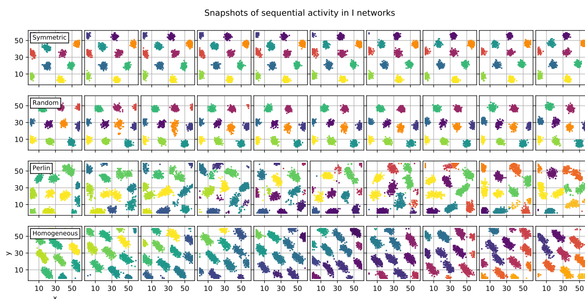
Figure S3: Snapshots of the spiking activity in I-networks for the four different configurations. Each row show the temporal evolution of the network activity for a different configuration. Each panel shows the activity of inhibitory neurons observed over a time window of 100 ms (disjoint windows), rendered in the two-dimensional network space. Each dot in a panel shows a spike of the neuron located at that grid point. Neurons are colored to identify individual spatio-temporal activity sequences (STAS). In each row, spikes rendered in the same color belong to the same STAS. Spikes that were not part of an STAS are not shown for clarity of presentation.
