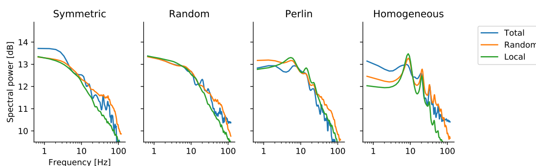
Figure S5: Power spectra of EI-network activity in different spatial inhomogeneity configurations. Power spectra of summed spiking activities of excitatory neurons (binwidth = 4ms), with different traces referring to the source of the data: the z-score of the spiking activity of the entire network population (blue trace), of 100 randomly selected neurons from the entire network (orange trace), and of the neurons located in a 10 \times 10 region in the network (green trace). The spectral power in all network models peaked at approx. 60 Hz (gamma-band oscillations). Additionally, in network models with homogeneous and Perlin configurations, an additional, weak low-frequency peak, at around 4-6 Hz, appeared.
