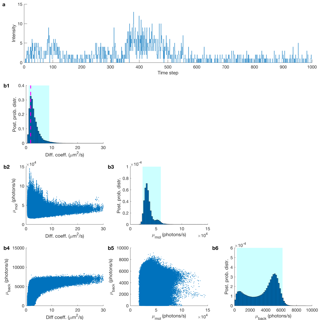
FIG. S7. Estimated joint posterior probability distribution. (a) Experimental fluorescent intensity trace used in Fig. 5b4 with a length of 1000 data points and time step 100 \mu\text{s} . (b1) The posterior of the diffusion coefficient. The FCS estimate is shown by a magenta dashed line. (b2) The joint probability distribution of the diffusion coefficient and the molecular brightness. (b3) The posterior probability distribution of the molecular brightness. (b4) The joint probability distribution of the diffusion coefficient and the molecular brightness. (b5) The joint probability distribution of the molecular brightness and background photon emission rates. (b6) The posterior probability distribution of the background photon emission rate and the 95% confidence intervals of the posteriors are highlighted in cyan. The experimental fluorescent intensity trace produced is with a concentration of 1 nM of Cy3 in a 94% glycerol/water mixture.
