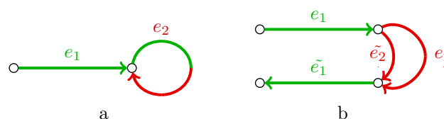
Figure 2: Examples of chimeric connections in the de Bruijn graph typical for transcriptome assembly. Red and green indicate erroneous and correct sequences respectively. (a) A chimeric loop (edge e_2 ) connecting end of the correct transcriptomic edge e_1 with itself. (b) An example of chimeric hairpin, where erroneous edge e_2 connects a correct edge e_1 with its reverse-complement copy \tilde{e}_1 . Since e_2 connects a vertex and its reverse-complement, \tilde{e}_2 (the reverse-complement of e_2 ) also connects these two vertices.
