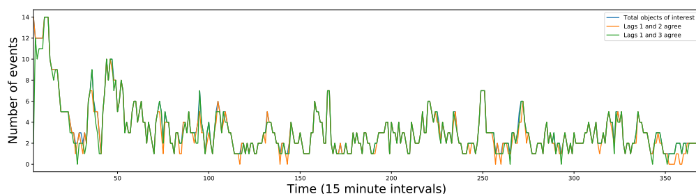
Fig 12. Dis/agreement between lags: Lag-1 identifiers for objects of interest (excluding single-frame detections) are compared with identifiers assigned by \lambda_\tau : \tau \in \{2, 3\} transformations for objects that are older than \tau . We counted 734 objects in a sample sequence. 42 \approx 6\% showed lag1-2 disagreements and excluding these, 29 \approx 4\% showed lag1-3 disagreements in specific frames.
