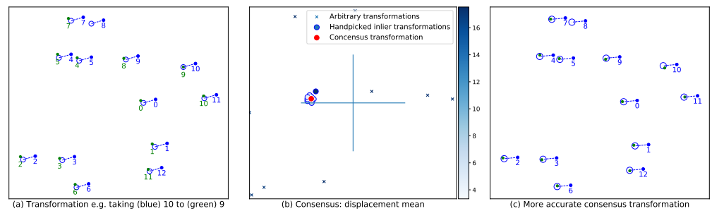
Fig 3. Translation sampling with k = 1 : Panel (a) shows an arbitrary translation between a sample point in V and a sample point in U . Panel (b) shows the displacement of many such translations from the origin and includes a “consensus” translation i.e. the average of the top ranked translations. Panel (c) illustrates that in this case, the consensus translation is better than the one in panel (a) making better matches between circles and green dots. In this case, while not discernible from the image, the consensus translation turns out to be better than any of the other sampled translations.
