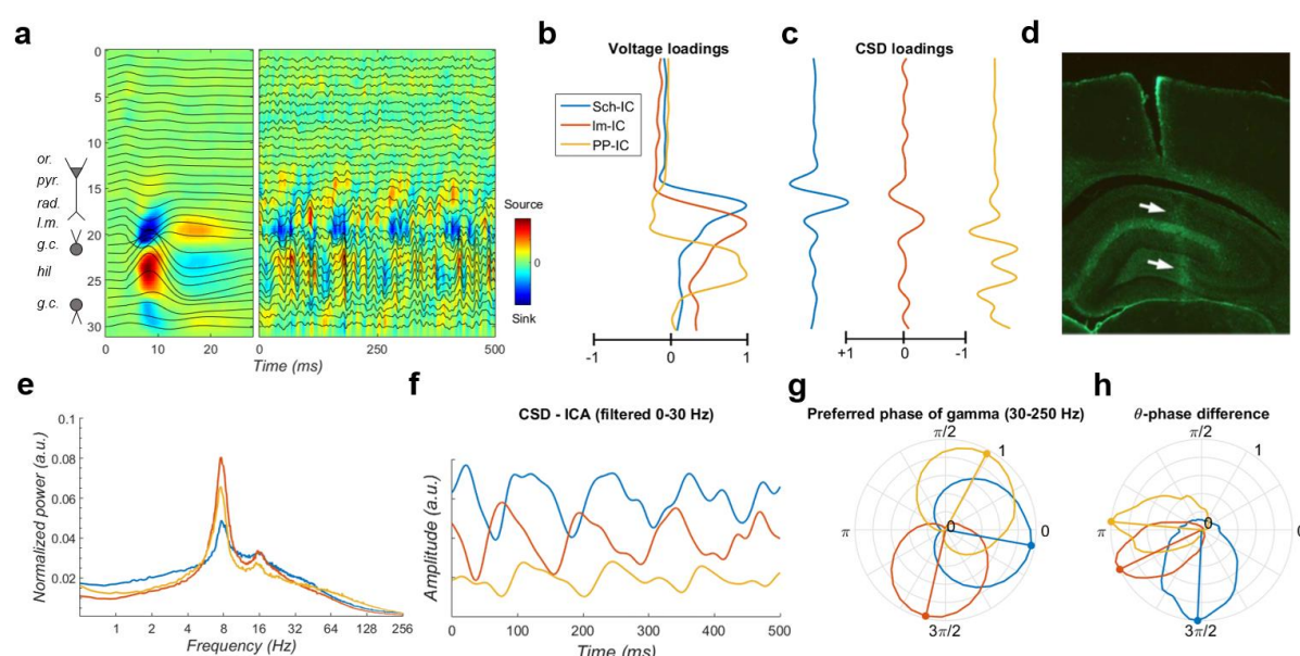
Figure 1. Layer-specific local field potentials (LFPs).
