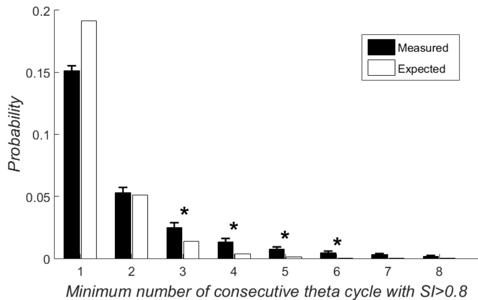
Figure S2: High synchronization epochs preferentially last three consecutive theta cycles. Each pair of bars compares the probability (mean \pm s.e.m) of, given a theta cycle with SI > 0.8 , find at least a certain number of consecutive cycles with strong synchronization ( SI > 0.8 ), and the probability expected by chance. The minimum number of cycles with a significant difference between measured and expected measurements is three theta cycles ( p < 0.001 , t-test), and goes on until six cycles ( p < 0.01/0.05/0.05 , respectively, t-test).
