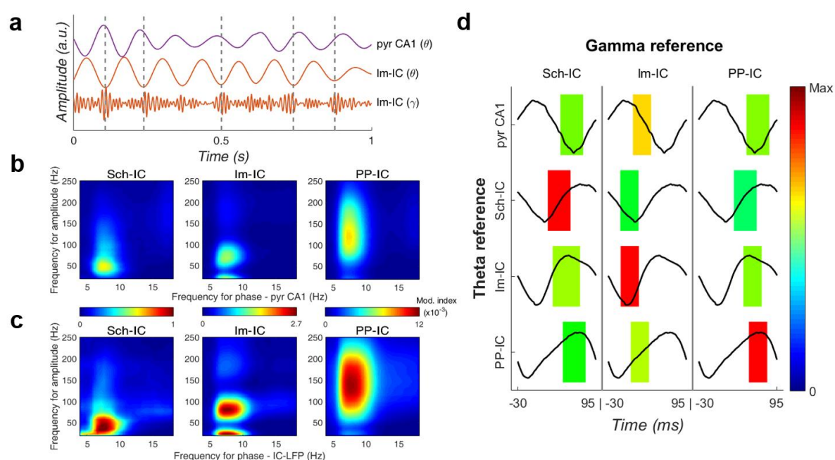
Figure 4. Theta-gamma coupling reflects layer-specific interactions.
