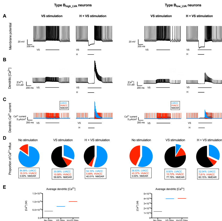
Figure 5: Effects of VS and H+VS stimulus protocols on membrane potential and [Ca^{2+}] in a dendritic compartment of a Type B high_LVA or Type B low_LVA MVN cell. The same stimulation protocols and analysis as in Fig. 3 are applied here. In the Type B high_LVA neuron the post-hyperpolarisation rebound firing and the dendritic Ca^{2+} influx were significantly greater than in the normal Type B neuron, while the Type B low_LVA neuron showed a much smaller rebound depolarisation and reduced dendritic Ca^{2+} influx than the normal Type B neuron. Note that because the types of neurons differ in LVA density, they have different basal calcium concentrations, and a direct comparison of absolute values between types of neurons is therefore difficult.
