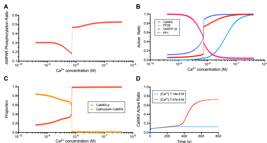
Figure 2: Dependence of AMPAR phosphorylation and relative activation ratios of key molecular species on [Ca^{2+}] . A. AMPAR phosphorylation ratio (phosphorylated AMPAR over total AMPAR) as a function of [Ca^{2+}] over the range 4 \times 10^{-10} M to 4 \times 10^{-7} M. For each data point the biochemical model was re-initialised and after reaching equilibrium the intracellular [Ca^{2+}] was stepped up to successively higher values (logarithmic scan of [Ca^{2+}] range, 151 simulations). Each simulation was run for 1600 s, to steady state. Note the initial dephosphorylation of AMPA receptors with increasing [Ca^{2+}] , which is followed by a switch to a large sustained increase in AMPAR phosphorylation when [Ca^{2+}] is increased above a threshold value for inducing long-term potentiation. B. Relative activation ratios (concentration of active molecules divided by total molecules) for CaMKII, PP2B, DARPP-32, and PP1 as a function of [Ca^{2+}] . C. The proportion of the two active CaMKII forms: CaMKII-p (phosphorylated CaMKII) and calmodulin-bound (non-phosphorylated) CaMKII as a function of [Ca^{2+}] . D. Time-course of activation of CaMKII over a period of 800 s, at two values of [Ca^{2+}] on either side of the threshold concentration.
