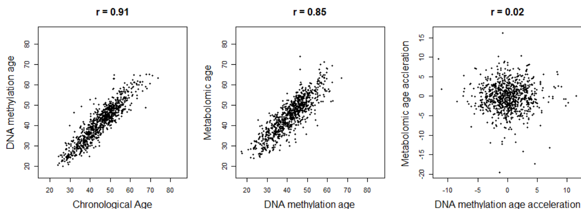
Figure 2: Relationships between different age measures. A. DNA methylation age plotted against chronological age. B: metabolic age plotted against DNA methylation age. C. MetAA plotted against DNAmethAA. Pearson's correlation coefficients ( r ) are shown
