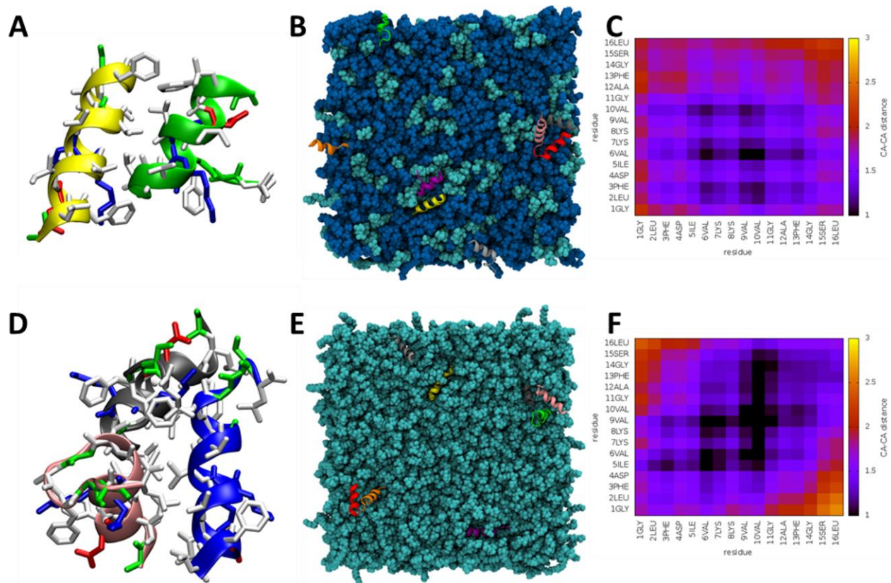
Figure 4. Interaction of aurein 2.5 with lipid bilayers. Examples of peptides aggregating as a dimer or a trimer are shown respectively for POPE/POPG (A) and POPG (D). Basic, polar, acidic and hydrophobic residues are coloured in blue, green, red and white respectively. The top view snapshot shows the tendency to aggregate for the eight peptides in POPE/POPG (B) or POPG (E). Heatmaps of average Ca-Ca distances for peptides in POPE/POPG (C) or POPG (F) show the stronger interactions that mediate assembly of aggregates
