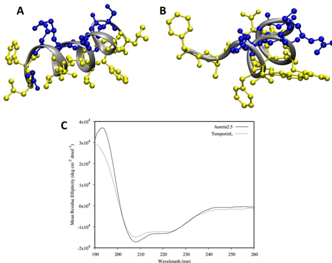
Figure 1. Three-dimensional structure for aurein 2.5 and temporin L. Structures were determined through ^1\text{H} -NOESY NMR spectroscopy in SDS-d25 micelles (peptide/detergent equal to 1/50). The figure shows the structure with the minimum RMSD, used as starting point in the MD simulations. The hydrophobic and hydrophilic residues are shown in yellow and blue for aurein 2.5 (A) and temporin L (B). CD spectra of the peptides in the same conditions used for NMR experiments (C).
