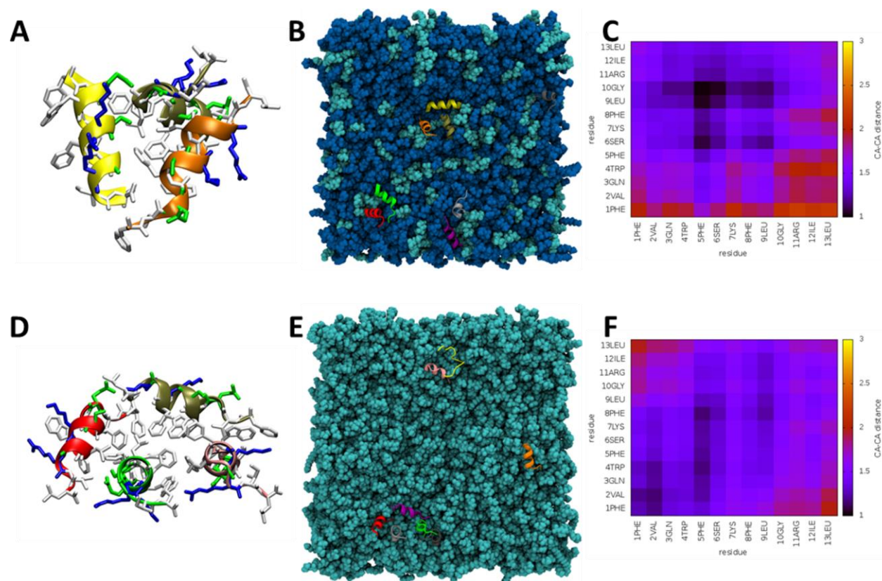
Figure 5. Interaction of temporin L with lipid bilayers. Examples of peptides aggregating as a trimer or a tetramer are shown respectively for POPE/POPG (A) and POPG (D). Basic, polar, acidic and hydrophobic residues are coloured in blue, green, red and white respectively. The top view snapshot shows the tendency to aggregate for the eight peptides in POPE/POPG (B) or POPG (E). Heatmaps of average Cα-Cα distances for peptides in POPE/POPG (C) or POPG (F) show the stronger interactions that mediate assembly of aggregates.
