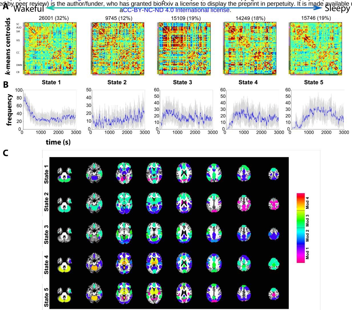
Figure 3: Cluster centroids from k-means clustering of dFNC window data for window size 30 (A) and the frequency of occurrence of each state in time (B). The standard errors for the frequency of occurrence were computed using 100 bootstrap resamples of the subject dFNC window data. (C) The modularity of the centroids is computed using the Louvain algorithm ("modularity_louvain_und_sign.m" function in the Brain Connectivity toolbox) resulting in three modules (Mod) for states 1,2 and 3 and four modules for states 4 and 5. The top 12 ICs with highest mean within module FC are depicted scaled by mean within module FC. Note that the weights (mean within module connectivity) are lower in states 1 and 5 compared to states 2, 3 and 4.
