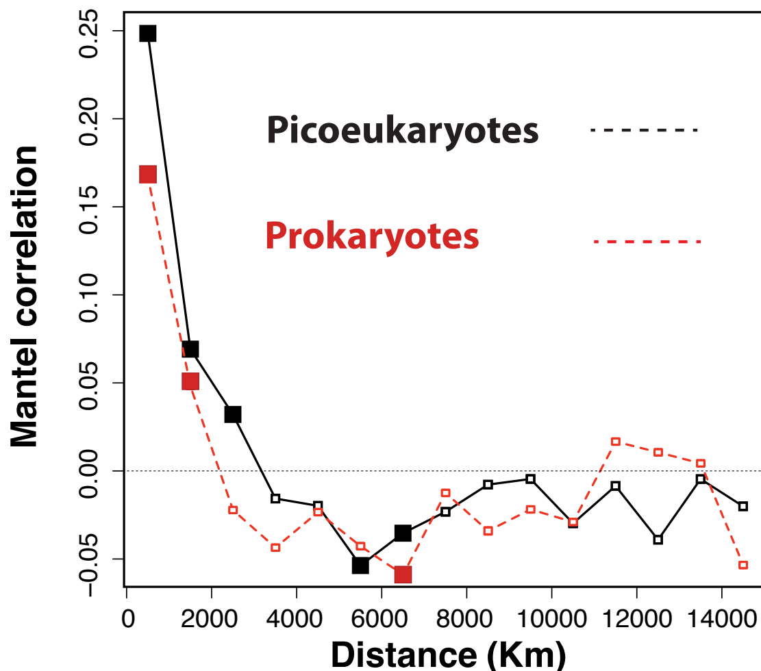
Figure 5. Decrease in community similarity with distance (distance decay). Mantel correlograms between geographic distance and \beta -diversity featuring distance classes of 1,000 km for both picoeukaryotes and prokaryotes. Coloured squares indicate statistically significant correlations ( p < 0.05 ). Note that \beta -diversity in picoeukaryotes displayed positive correlations with increasing distances up to ~3,000 km, while prokaryotes had positive correlations with distances up to ~2,000 km. Correlations tended to be smaller in prokaryotes than in picoeukaryotes, indicating smaller distance decay in the former compared to the latter.
