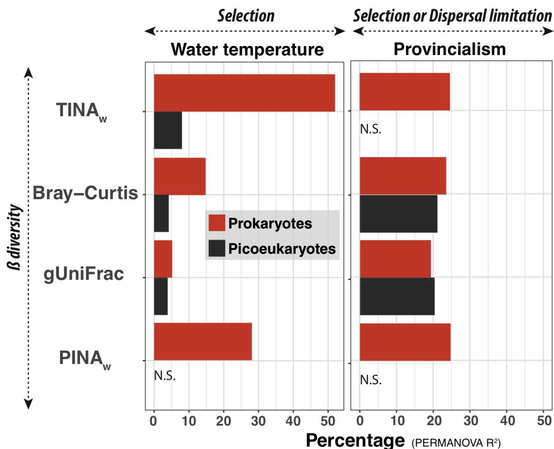
Figure 2. Water Temperature and Provincialism were the most important variables explaining the structure of the tropical and subtropical surface-ocean microbiome. Percentage of variance in picoeukaryotic and prokaryotic community composition (PERMANOVA R^2 ) explained by Water Temperature and Longhurst Provinces when using different \beta -diversity metrics. Figure based on the Meta-119 dataset (see Methods). TINA_w : TINA weighted, gUniFrac: Generalized Unifrac, PINA_w : PINA weighted. N.S. = Non-Significant. Note that TINA_w captures a significantly higher proportion of community variance than Bray-Curtis in prokaryotes.
