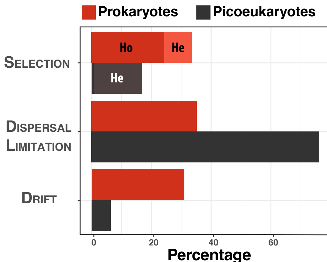
Figure 1. Relative importance of the processes shaping the tropical and subtropical sunlit-ocean microbiome. Percentage of the spatial turnover governed by different processes in prokaryotes and picoeukaryotes. Ho = Homogeneous selection, He = Heterogeneous selection (light red and light black).
