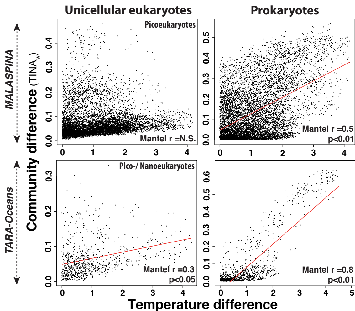
Figure 3. Temperature-driven selection affects species co-occurrences in prokaryotes but not in small unicellular eukaryotes. Community differences (Tina-weighted dissimilarities) vs. temperature differences (Euclidean distances) for both small unicellular eukaryotes and prokaryotes sampled during the Malaspina and TARA Oceans expeditions. NB: While only picoeukaryotes were contemplated in Malaspina (cell sizes <3 \mu\text{m} ), TARA Oceans data included pico- and nanoeukaryotes (cell sizes <5 \mu\text{m} ). Pico- and nanoeukaryotes from both expeditions (left panels) displayed low or no correlations between TINA w distances and temperature differences (Note Mantel test results in the figures). On the contrary, prokaryotes (right panels) had high to moderate
