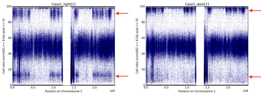
Figure 1 Case 1 B-allele plots. These figures show the expected diploid B-allele frequency bands at 0%, 50%, and 100% for the two fibroblast samples from case 1, light skin on the left and dark skin on the right. In addition, partial bands that do not span the length of the chromosome (see arrows), can be seen. These partial bands are present in the same regions of the chromosome in each sample.
