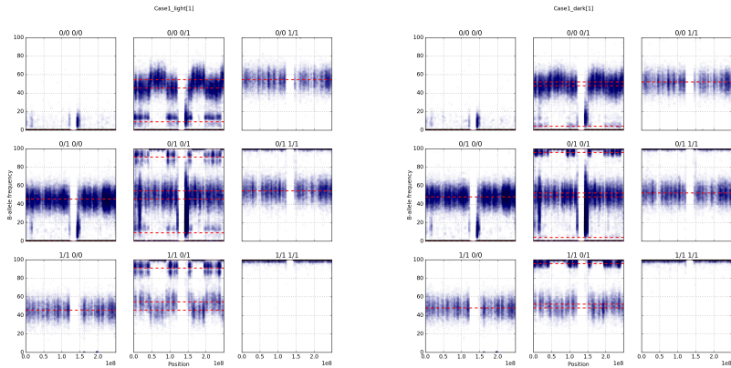
Figure 2 Case 1 Deconvoluted B-allele plots. These images show the B-allele frequencies for the light skin (left) and dark skin (right) fibroblasts from case 1 when split based on paternal and maternal genotype calls. Red dashed lines represent predicted B-allele frequencies derived from the formulae in Table 1. Note that each predicted frequency line resides roughly in the center of a band of observed frequencies.
