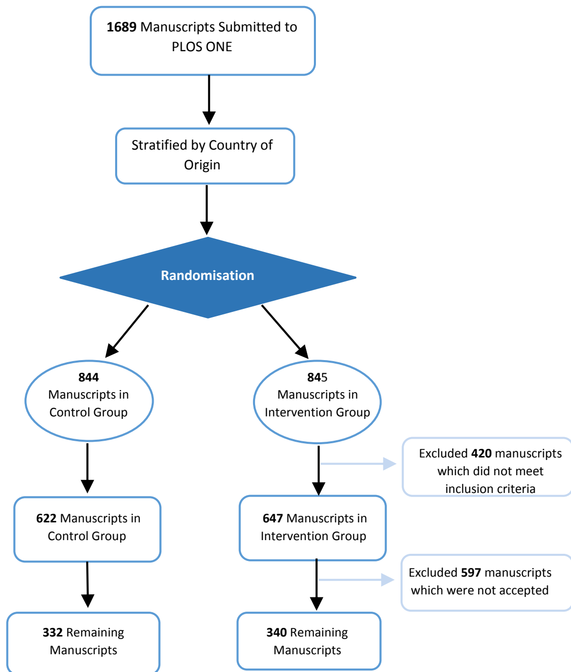
Figure 1: Manuscript processing
