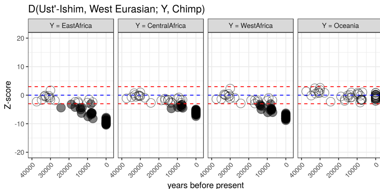
Figure 2 – Affinity of ancient and modern West Eurasian individuals to three African populations (left) and Oceanians (right). Z score values for D(\text{Ust'-Ishim, } X; \text{ African population or Oceanians, Chimp}) , where X is a series of European individuals over time. Negative Z-scores indicate that an individual X is significantly closer to a population in the third position of the D statistic than Ust'-Ishim is. Assuming all non-Africans share a common ancestor after the split from an African lineage, this can be interpreted as evidence of gene-flow between Europeans and Africans over time and no such gene flow between Europeans and Oceanians.
