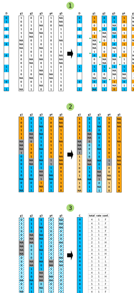
Supplementary Fig. 5: High-resolution consensus haplotype assembly. (g1, ..., g5 are the 5 gamete cells; 0 and 1 represent the two alleles that are arbitrarily assigned for a hetSNP locus; D represents draft haplotype and C represents consensus haplotype; In the table of consensus haplotype, 'total' is the total number of cells with observed genotypes at a locus, 'rate' is the ratio of cells supporting the haplotype, and 'conf.' is the confidence of haplotype phasing for each hetSNP, i.e. , F indicates that the hetSNP is in the framework, L denotes low-confident phasing, whereas H represents high-confident phasing that is supported by at least 2 gametes and the ratio of cells supporting the haplotype is greater than 0.6; Green triangles mark the HCPs inferred by comparing genotypes in each gamete cell with those in the draft haplotype. The two colors of background indicate the two haplotypes in each gamete, and regions with grey background are unsolved haplotype regions; The regions with slash represent the haplotypes after flipping.)
