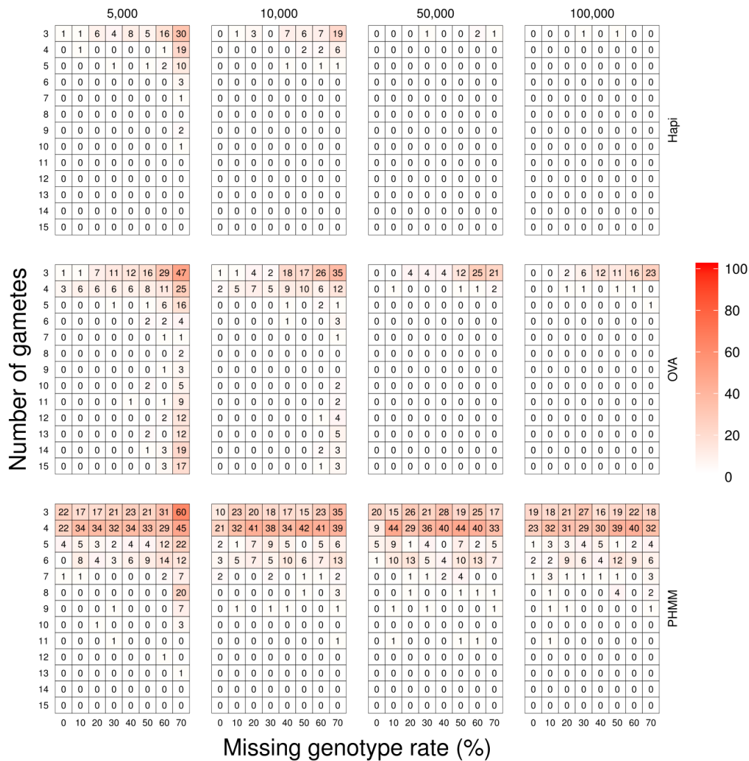
Fig. 2: Performances of three methods (Hapi, OVA, and PHMM) in the simulated dataset for 5,000 to 100,000 hetSNPs per chromosome. The number in each heatmap grid denotes for how many times out of the 100 replicates the haplotypes are incorrectly inferred in that scenario.
