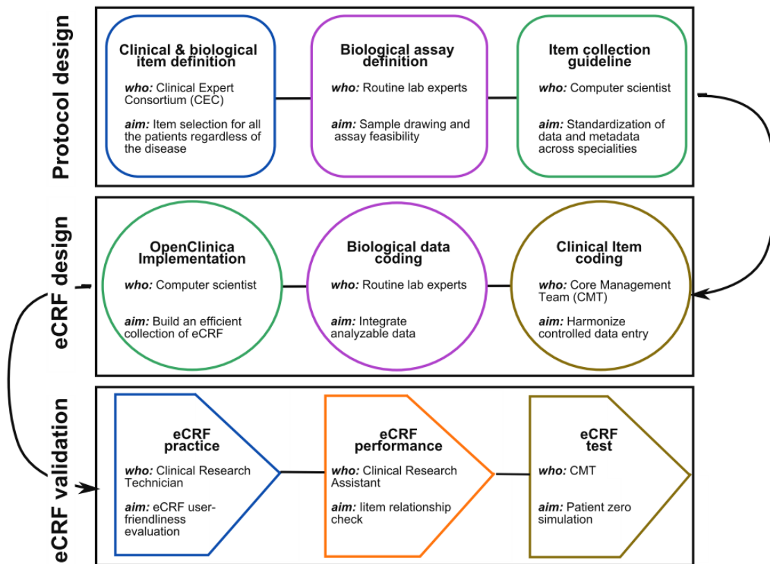
Figure 2: eCRF workflow
