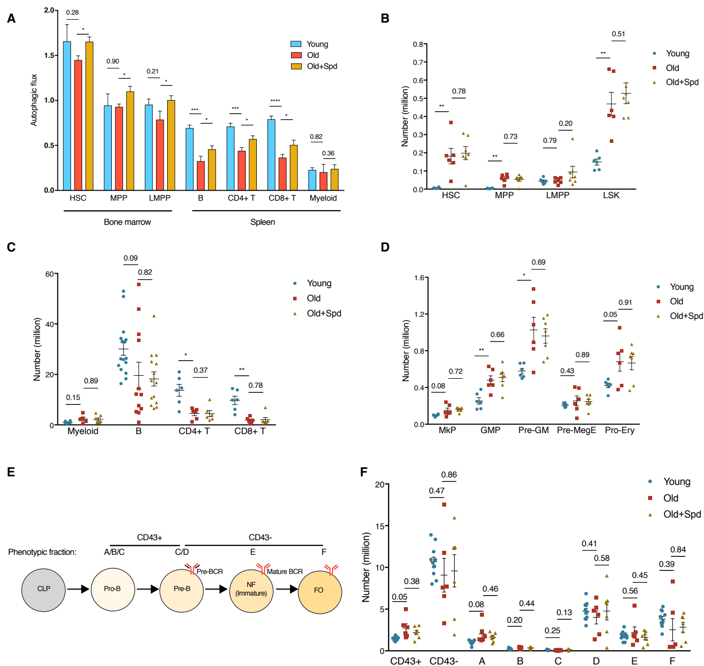
Figure 1 Spermidine induces autophagy in vivo but does not affect hematopoiesis in old mice.
