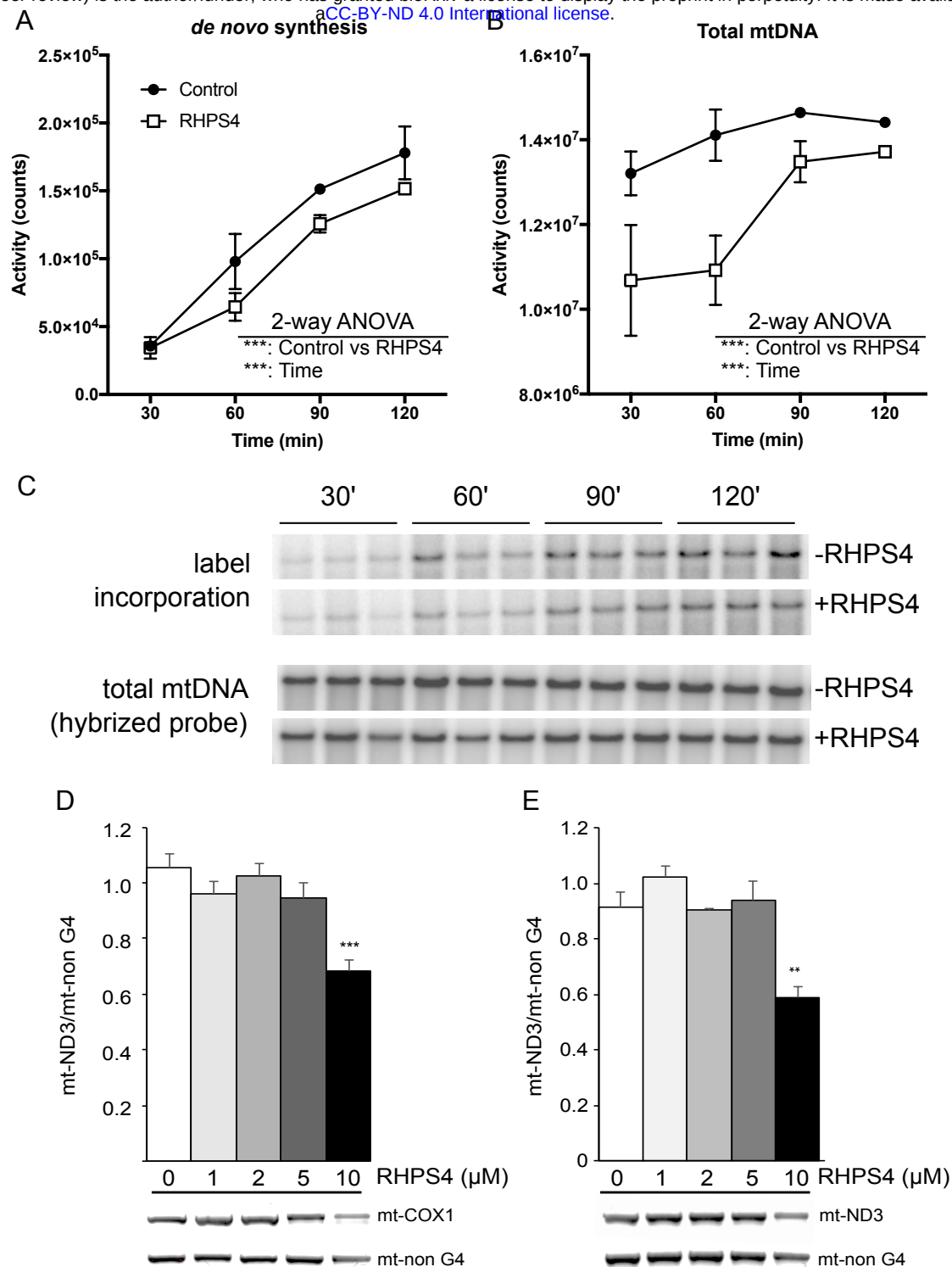
Figure 2. RHPS4 inhibits mtDNA replication or polymerization in vitro. (A,B) DNA replication in isolated mouse liver mitochondria with or without 2 μM RHPS4. (A) Radiolabel incorporation into full-length mtDNA across 30-120 min timecourse. (B) Total full-length determined by hybridization probing and autoradiography. (C) Raw radiographic images of full length mtDNA. (D,E) PCR stop assay using untreated HeLa cellular DNA amplifying mt-COX1 (G4 amplicon; D) or mt-ND3 (G4 amplicon; E) and mt-non G4 (no G4 in amplicon). Amount of RHPS4 in PCR reaction as indicated. Data are shown as mean \pm SEM (n=3). P-values determined by 2-way (A,B) or 1-way ANOVA (D,E; * <0.05 ; ** <0.01 ; *** <0.001 ).
