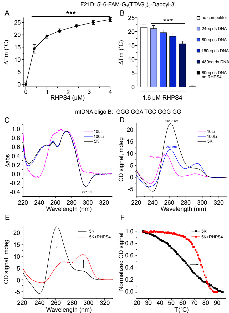
Figure 4. RHPS4 is a G-quadruplex ligand that stabilizes antiparallel structures in G4-forming mtDNA sequences. (A) FRET-melting profile of 0.2 μM F21D, a fluorescently labeled G4-forming human telomeric DNA, in the presence of increasing concentration of RHPS4. (B) FRET-melting competition assay showing the inability of dsDNA to compete with F21D for RHPS4 binding. Negative control consists of 0.2 μM F21D, 80 eq of dsDNA and no ligand. P-values for Panel A and B were calculated by one-way ANOVA with Dunnett's posthoc analysis: ***<0.001. (C) The UV-VIS TDS characteristic negative peak at 295 nm supports G4 structure formation of oligo B in 10Li, 100Li, or 5K buffer. (D) CD spectra of 5 μM mtDNA sequence oligo B in the 10Li, 100Li, or 5K buffer. Parallel and antiparallel G4 character is detected at ~264 nm and ~295 nm, respectively. (E) CD spectra of 5 μM mtDNA sequence oligo B in the presence (red lines) or absence (black lines) of 10 μM RHPS4 in 5K buffer. (F) CD melting curve for oligo B, with or without RHPS4. Signal was monitored at 260 nm for oligo B or 295 nm in the presence of RHPS4.
