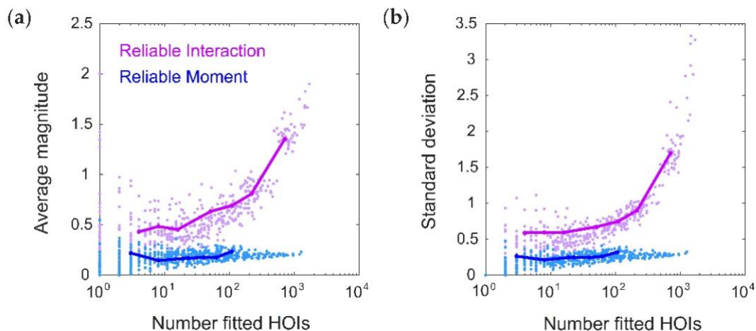
Figure 3. The Reliable Moment (RM) infers fewer strong, spurious higher-order interactions. (a) Average magnitude of all fitted higher-order interaction parameters as a function of the number of fitted higher-order interactions, shown for both the Reliable Interaction (RI; magenta) and RM (blue) models. Note that all higher-order interactions should have magnitude 0. Points represent 50 random ground-truth models (i.e., random interaction parameters), each of which is fitted 20 times with varying threshold parameters (see Methods). Solid lines indicate the RM and RI fits to a specific example ground-truth model. (b) Same as (a) but for standard deviation.
