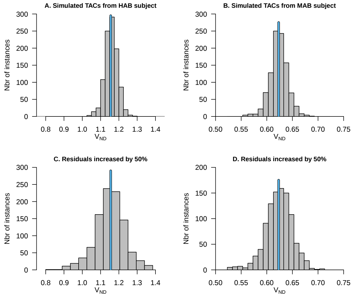
Figure 1: Estimation of V_{ND} from simulated time-activity curves using SIME. In each plot, 1000 noise instances have been created and added onto a set of noise-free model curves obtained from a HAB subject (A and C) or a MAB subject (B and D) randomly selected from the KI [ ^{11}\text{C} ]PBR28 database. In C and D the noise have been amplified by a factor of 1.5. The blue vertical lines indicate the “true” value of V_{ND} .
