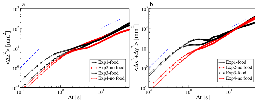
Figure 4: For the four different experiments, mean square displacement (a) along the vertical ( z ) direction and (b) in the horizontal ( x, y ) plane. The dashed and dotted lines are guide to the eye corresponding to a ballistic, \langle \Delta r^2(\Delta t) \rangle \propto t^2 , and diffusive, \langle \Delta r^2(\Delta t) \rangle \propto t , behaviour, respectively.
