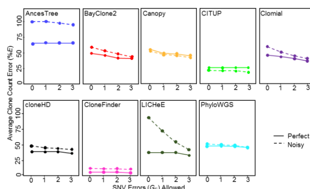
Figure 4: Average clone count errors in the analysis of G7 datasets. Average of the proportion of correct clones not found (%E C ) and incorrect clones found (%E I ), i.e., %E, were computed when allowing for one or more SNV assignment errors ( G_E ). A solid line is for datasets without read count errors (perfect), and a dashed line is for datasets with read count errors (noisy).
