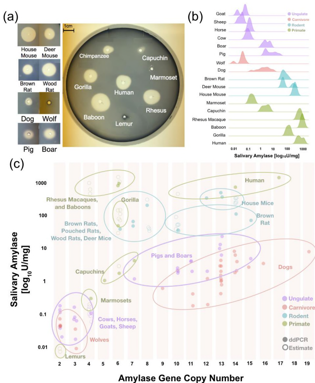
Figure 3: Salivary amylase activity and relationship to gene copy number. (a) A representative starch lysis assay plate showing the activity levels of amylase in the saliva of various mammalian species. (b) Density plots showing salivary amylase activity in different species. Full dataset can be found in Table S1 . (c) Correlation of amylase activity and gene copy number in multiple different species. Data obtained by direct genotyping are represented by filled circles, while data estimated from reference genomes or through genotyping of other samples from the same species are represented by empty circles.
