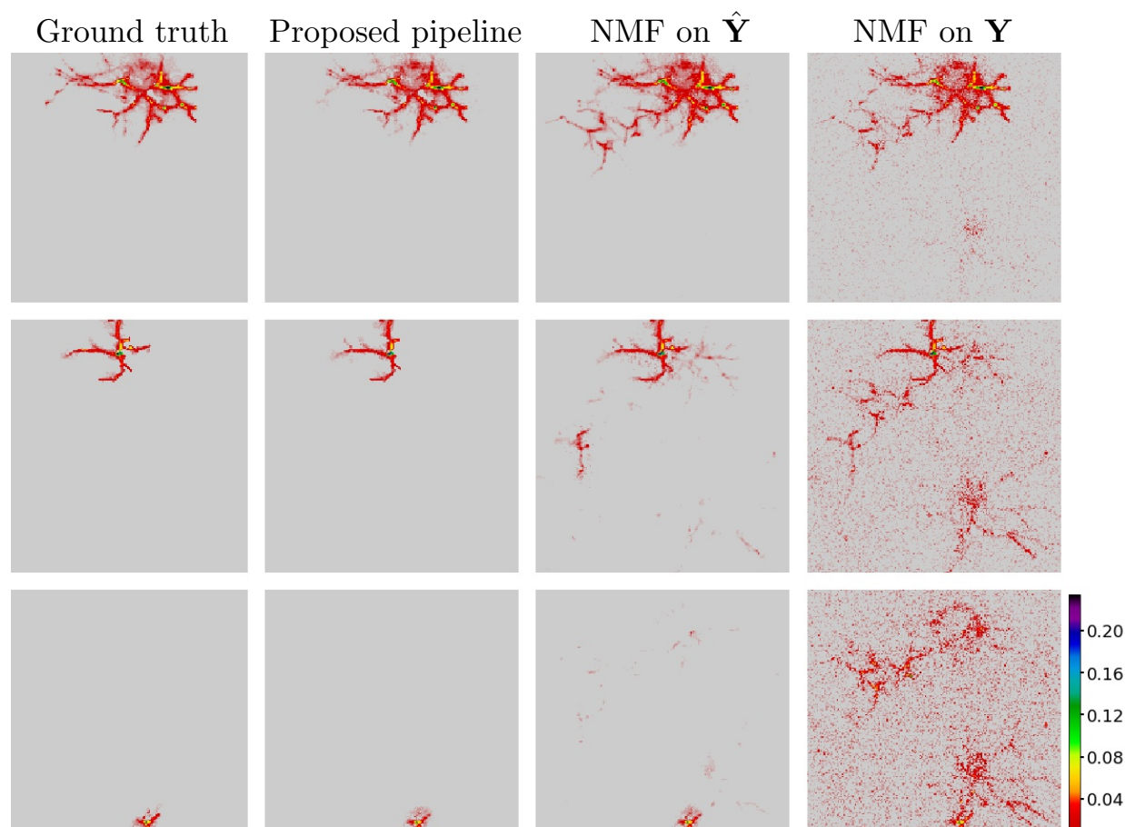
Figure 16: Comparison to simulated ground truth based on Bessel dendritic imaging data. Spatial components are arranged as in the previous figure, with the addition of ground truth components shown in the first column. Note that the proposed pipeline recovers the ground truth simulated components much more accurately than do the sparse NMF baseline approaches.
