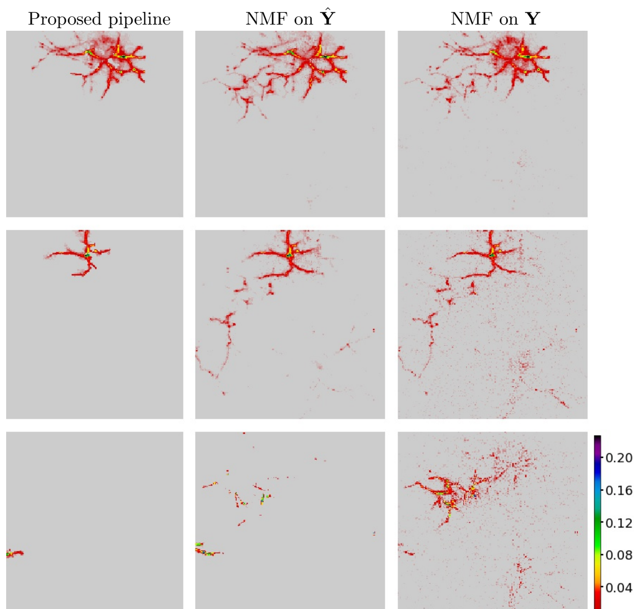
Figure 15: Comparison of spatial components extracted from Bessel dendritic imaging data. Each row shows best-matching components extracted by our proposed method (first column), sparse NMF on denoised data \hat{Y} (second column) and sparse NMF on raw data Y (third column). See the Bessel dendritic imaging demixing video for further details. The proposed pipeline extracts components that are significantly more localized and less noisy than the components extracted by sparse NMF; also note that denoising helps sparse NMF extract cleaner spatial components.
