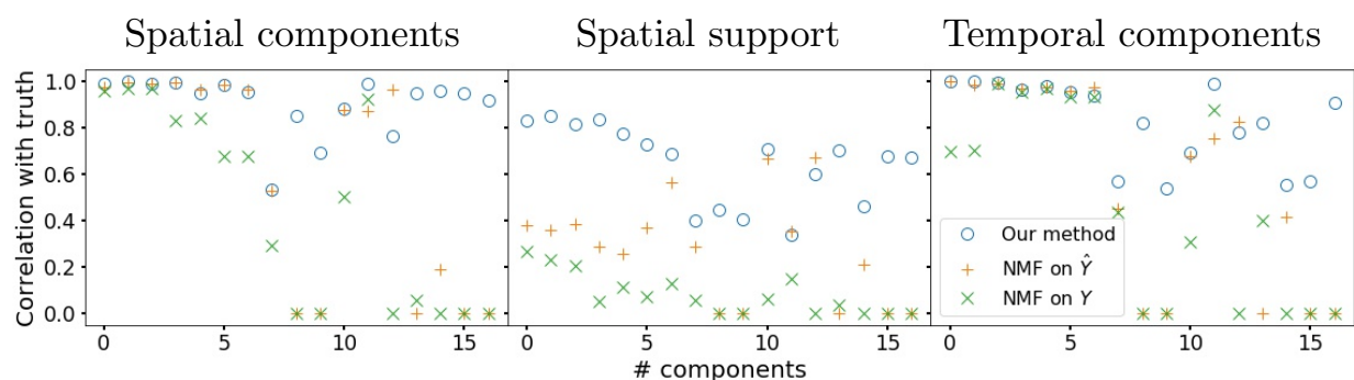
Figure 17: Quantification of comparisons on simulated Bessel dendritic imaging data. Components are ordered by brightness; top 17 brightest components shown here. First column shows the correlation between true vs spatial components estimated by proposed pipeline ( \circ ), sparse NMF on \hat{Y} ( + ), and sparse NMF on Y ( \times ). Second column shows the correlation between the supports of the true and estimated spatial components. Third column shows the correlation between the true vs estimated temporal components. (The baseline NMF approaches missed some dimmer, weaker neurons, so the corresponding symbols are set to zero here.) Note that components extracted by proposed pipeline typically have higher correlation with true components than sparse NMF baseline approaches.
