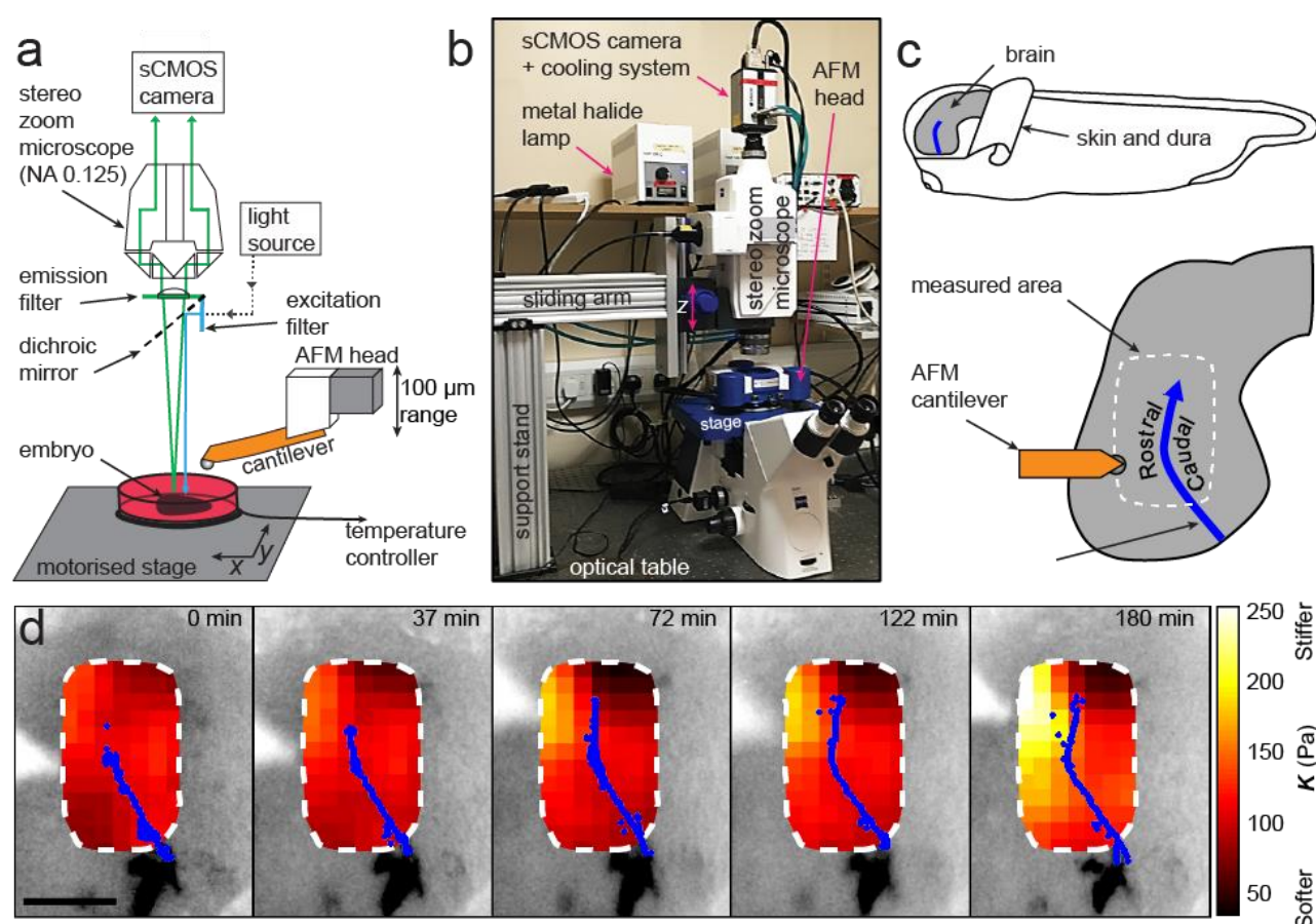
Figure 1: Combined time-lapse in vivo AFM (tiv-AFM). (a) Schematic (not to scale) and (b) photograph of the experimental setup. An AFM with 100 \mu\text{m} z-piezo range is positioned above a temperature-controlled sample chamber containing the specimen. A custom-fit fluorescence zoom stereomicroscope with a long (114 mm) working distance and NA 0.125 objective, connected to a high quantum-efficiency sCMOS camera, is mounted on a custom-built support stand above the AFM head optimised for trans-illumination. The specimen is moved by a motorised x/y stage to allow AFM-based mapping of large areas. (c) Schematic of a Xenopus embryo, showing how the brain is prepared for tiv-AFM (top) and close-up of the brain (bottom) showing the approximate region measured, within which optic tract (OT) axons (blue) turn caudally. (d) Time-lapse stiffness maps obtained from a tiv-AFM experiment, showing outlines of fluorescently labelled OT axons (blue) and processed AFM-based stiffness maps (colour maps) overlaid on images of the brain. Colour maps encode the apparent elastic modulus K , a measure of tissue stiffness, assessed at an indentation force F = 10 nN. The time in minutes on each frame is taken from the timestamp of the first measurement in each successive stiffness map; the corresponding overlaid fluorescence images were obtained simultaneously. AFM measurement resolution, 20 \mu\text{m} ; scale bar, 100 \mu\text{m} .
