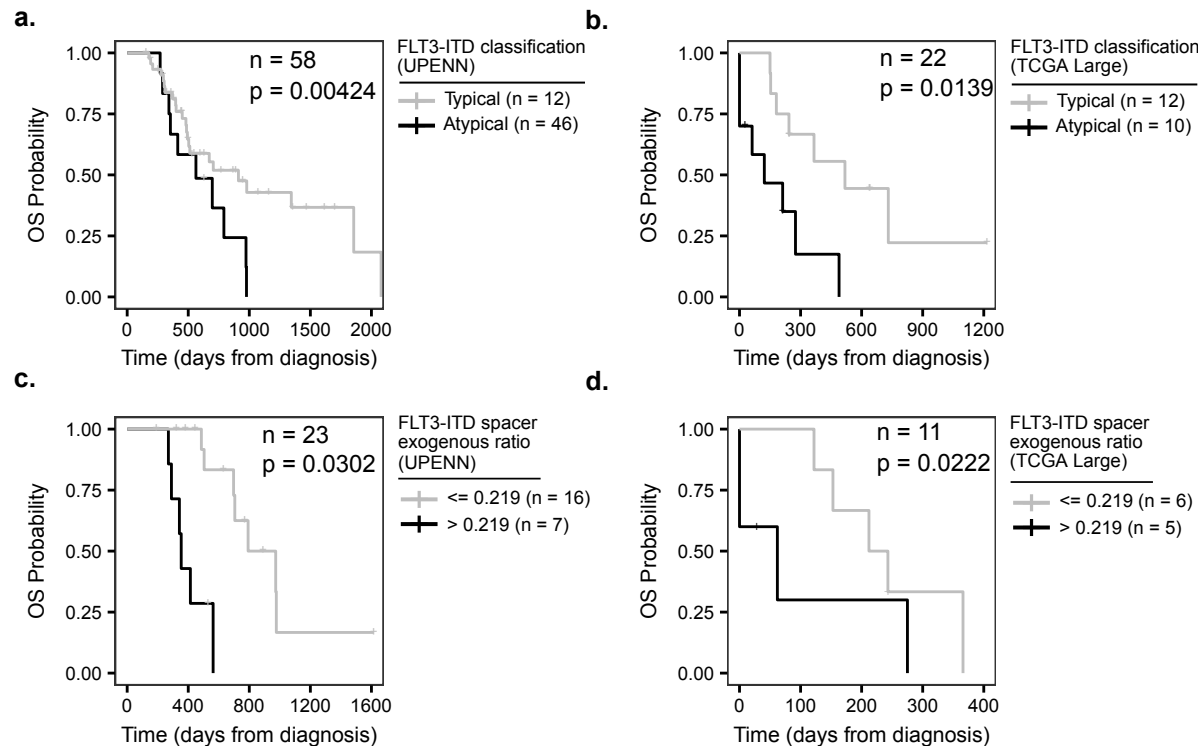
Figure 5. Correlation between ITD features and overall survival for the FLT3i-treated
