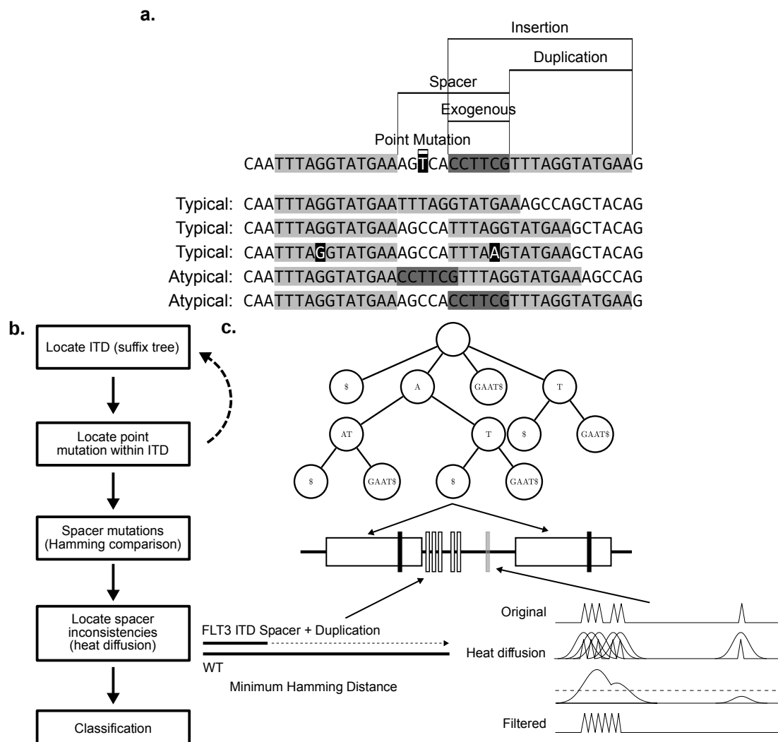
Figure 1. Schematic of ITD classification definition and HeatITup algorithm. a) Schematic of potential typical and atypical ITD mutations with marked duplication, spacer, and exogenous nucleotides. First sequence: structure of ITDs. Remaining sequences are examples of typical and atypical ITDs. Top to bottom: Duplication with no spacer; Duplication with spacer; Duplication with spacer and a point mutation; Duplication with entire spacer exogenous to exon; Duplication with part of spacer exogenous to exon. Light gray: duplicated, black: point mutation, dark gray: exogenous sequences. b) Outline of the HeatITup algorithm. c) Schematic of HeatITup modules and their function to analyze an ITD mutation. In this schematic, the FLT3 locus ITD sequence (middle, black horizontal line) is composed of the repeated substring (duplication, in large white boxes), a point mutation within the duplication (vertical black bars), a point mutation within the spacer (vertical gray bar), and exogenous nucleotides (vertical white
