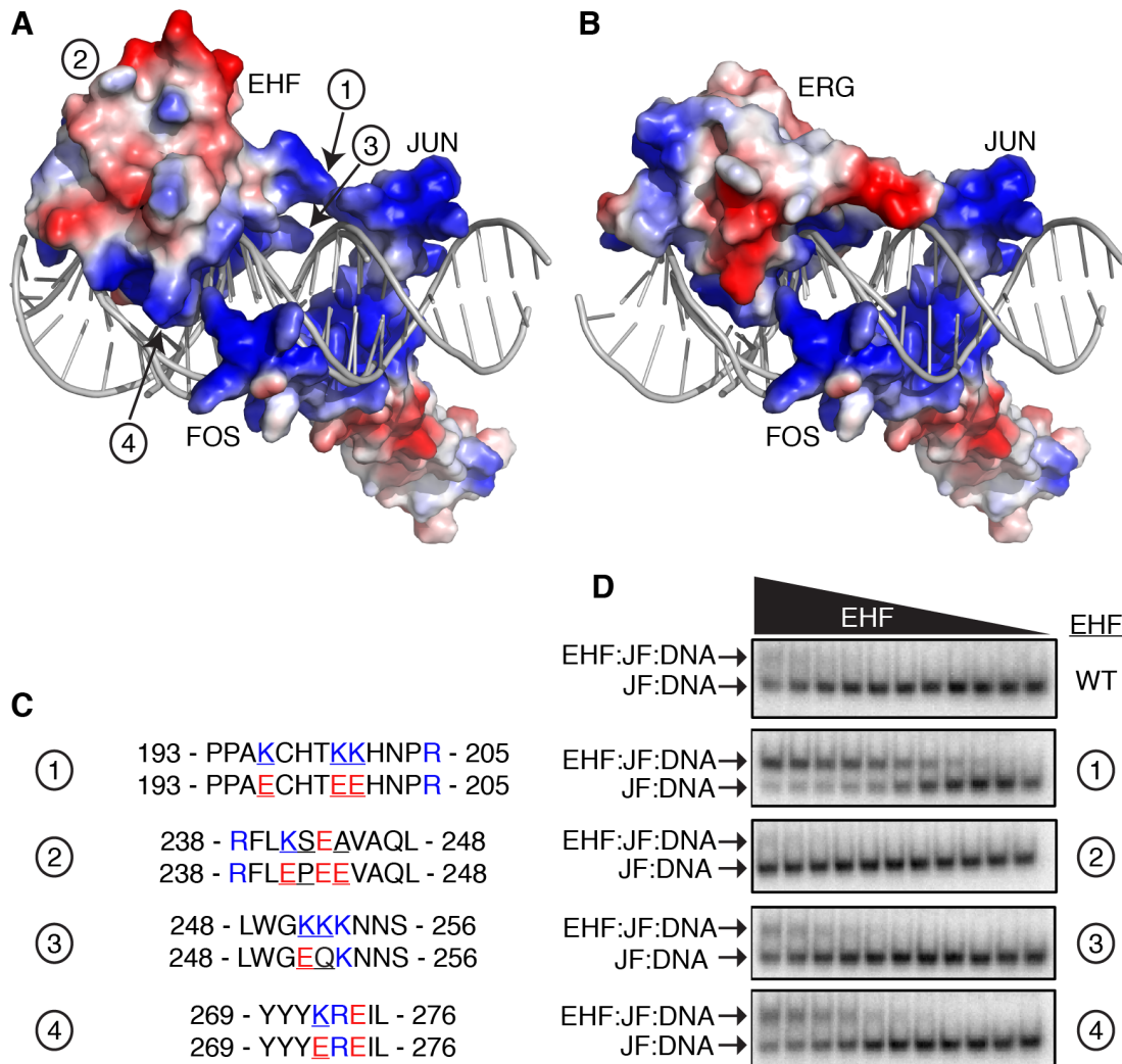
Figure 5. Positively-charged residues near the JUN-FOS interface are important for anticoooperative binding of EHF and JUN-FOS. Structural model of EHF A , and ERG B , binding to an ETS-AP1 composite DNA sequence with JUN-FOS. EHF, ERG, and JUN-FOS are shown in surface mode and colored according to electrostatic potential (red, negative; blue, positive). Regions of EHF that were subsequently mutated are labeled 1 – 4. Note that EHF residues 193-204 are not present in this structure. C , Listing of EHF residues that were mutated. Circled numbers 1 – 4 correspond to the regions labeled in A . The top and bottom sequences indicate the native and mutated residues, respectively. Residues are colored according to charge, as in A . D , Portions of EMSAs showing EHF wildtype (WT) and mutants bound in the presence of JUN-FOS on an ETS-AP1 site. EHF was serially diluted in twofold increments. Bands corresponding to JUN-FOS bound to DNA (JF:DNA) as well as EHF and JUN-FOS bound to DNA (EHF:JF:DNA) are labeled. See Fig. S6 and Table S6 for further quantification of EMSAs.
