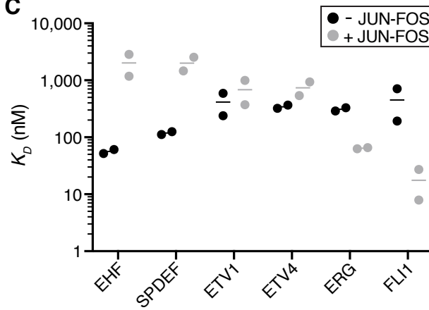
Figure 1. JUN-FOS differentially influences the DNA binding of ETS factors to AP1-ETS composite sites. A , Representative phosphorimages of electrophoretic mobility shift assays (EMSAs) for EHF (left), ETV4 (middle), and FLI1 (right) binding to the UPP promoter DNA duplex. ETS titrations were performed with DNA alone (top), and with nearly saturating JUN-FOS bound to the DNA (bottom). The higher band for EHF corresponds to two EHF molecules bound to the DNA duplex, as previously observed for similar ETS factors (17). B , Binding isotherms for EHF binding to UPP DNA in absence (black), and presence (gray) of JUN-FOS. Each data point is the mean from two experiments. C , K_D values for ETS factors binding to UPP DNA without (black) or with (gray) JUN-FOS. The bar indicates the mean of the two experiments (filled circles). See Fig. S1 and Table S1 for quantification of equilibrium dissociation constants ( K_D ) from EMSAs.
