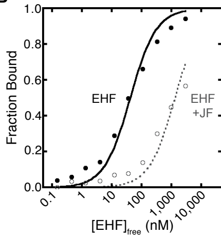
Figure 1. JUN-FOS differentially influences the DNA binding of ETS factors to AP1-ETS composite sites. A , Representative phosphorimages of electrophoretic mobility shift assays (EMSAs) for EHF (left), ETV4 (middle), and FLI1 (right) binding to the UPP promoter DNA duplex. ETS titrations were performed with DNA alone (top), and with nearly saturating JUN-FOS bound to the DNA (bottom). The higher band for EHF corresponds to two EHF molecules bound to the DNA duplex, as previously observed for similar ETS factors (17). B , Binding isotherms for EHF binding to UPP DNA in absence (black), and presence (gray) of JUN-FOS. Each data point is the mean from two experiments. C , K_D values for ETS factors binding to UPP DNA without (black) or with (gray) JUN-FOS. The bar indicates the mean of the two experiments (filled circles). See Fig. S1 and Table S1 for quantification of equilibrium dissociation constants ( K_D ) from EMSAs.
