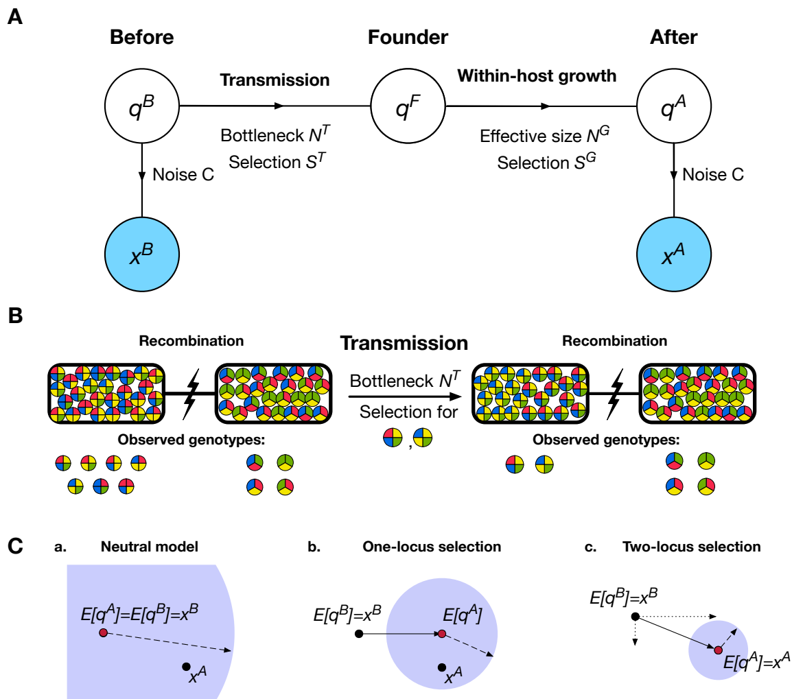
Figure 2. A. Basic model of transmission. A set of haplotypes exists at frequencies q^B from which a noisy observation x^B is made. During a transmission event, a total of N^T viruses are transferred under the influence of selection S^T , establishing an infection in the next host described by q^F . Growth of the viral population within the host then occurs to produce the population q^A , influenced by genetic drift (characterised by the effective population size N^G ) and selection S^G . Sampling of the final population gives the second observation x^A . B. Regions of the genome which are separated by recombination or reassortment are used to distinguish the effects of selection and a population bottleneck. Here, genetic diversity is reduced in one region but not in another; the preservation of diversity in the second region attributes this change to the action of selection on the first, rather than a shared population bottleneck. C. Models of neutrality and selection are compared, as illustrated in this simplified diagram. Black dots represent observations x^B and x^A while the red dot indicates the inferred expected position of q^A . The solid line joining these (b,c) indicates the inferred action of selection, with dotted lines showing components of this vector (c). The blue circle represents the optimised variance in the position of q^A ; the length of its radius, shown as a dashed line, is inversely related to the bottleneck size. In the neutral case, the difference between observations is explained by the bottleneck alone. More complex models of selection fit q^A more closely to x^A and with reduced variance, giving higher inferred values of N^T .
