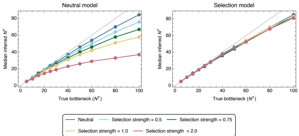
Figure S2. Median inferred bottleneck size from data simulating neutral transmission and transmission with a single locus under selection of magnitude \sigma \in \{0, 0.5, 0.75, 1.0, 2.0\} . Inferences were made using either a neutral model, in which the effect of selection was assumed to be zero, or a selection model, which allowed scenarios involving selection to be identified. Median inferences are shown from 100 simulations, each involving three replicate transmission events, for each datapoint.
