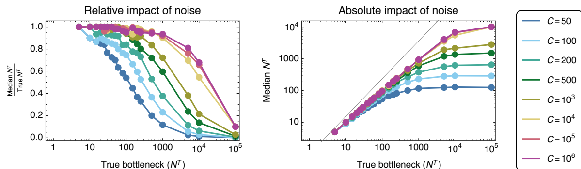
Figure 3. Influence of sequencing noise upon the ability to infer a population bottleneck size from genome sequence data. Median inferred bottlenecks are shown, calculated on the basis of 200 replicate simulations for each point. In the left-hand plot, a value of 1 indicates a correct bottleneck inference; in the right-hand plot, the absolute inferred bottleneck size is shown. Simulations were conducted under the assumption of selective neutrality, with no attempt to infer selection from the data.
