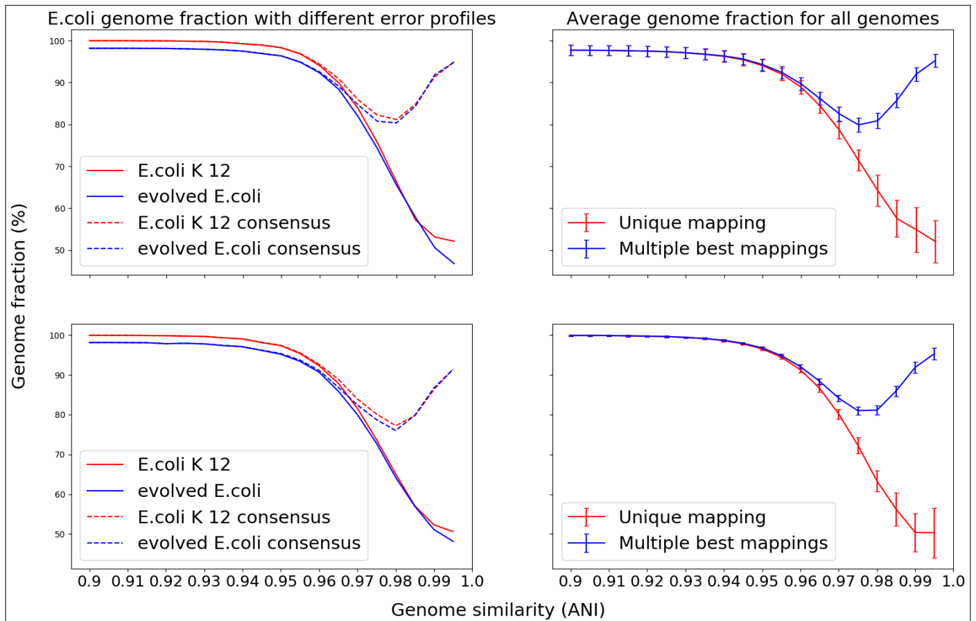
Fig. 4. Genome fraction calculated using unique or multiple best mappings in case of ties to the community genome collection. Left: Genome fraction for the E. coli assembly created by MEGAHIT from error-free reads (top) and with ART CAMI error profile (bottom). Right: Average genome fraction and standard deviation for all original 152 iToL genomes created by MEGAHIT from error-free reads (top) and with ART CAMI error profile (bottom). Error bars denote 1x standard deviation.
