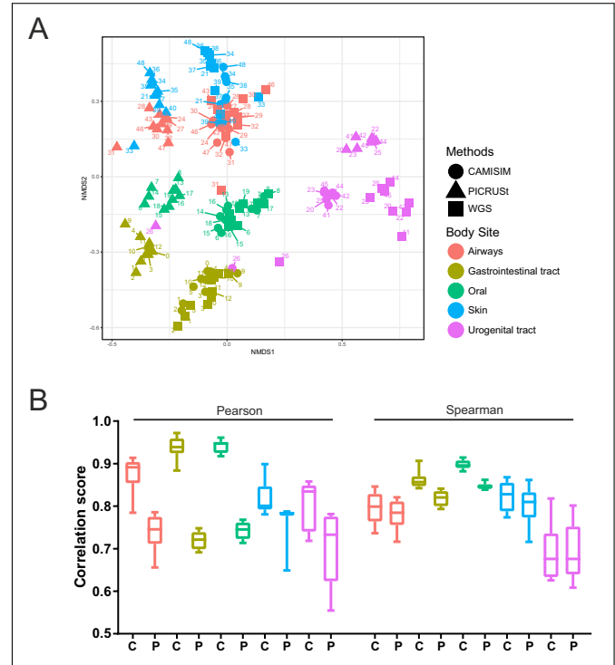
Fig. 5. Comparison of CAMISIM and PICRUSt functional profiles for different body sites. (A) NMDS ordination of the functional predictions of individual samples by the different methods. The different body sites are color-coded and labeled with their sample number. The original WGS is denoted by squares, the CAMISIM result as circles and the PICRUSt result as triangles. (B) Mean and standard deviation of Pearson and Spearman correlation to original WGS samples per body site. C: CAMISIM; P: PICRUSt.
