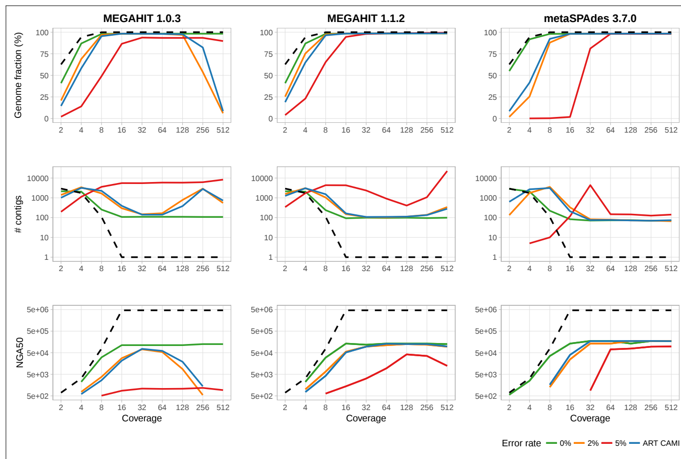
Fig. 3. Coverage dependent assembly performance for MEGAHIT and metaSPAdes. Shown are the metrics, from top to bottom: Genome fraction in %, number of contigs, and NGA50 (as reported by QUAST [51]), for 0%, 2%, and 5% uniform error rate, and with the ART CAMI error profile compared to the best possible metrics (gold standard) on the ART CAMI profile (dashed black).
