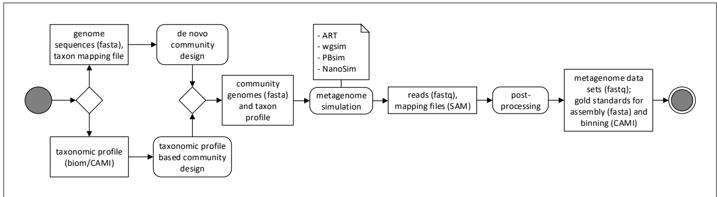
Fig. 1. UML diagram of the CAMISIM workflow. CAMISIM starts with the “Community Design” step, which can either be de novo , requiring a taxon mapping file and reference genomes or based on a taxonomic profile. This step produces a community genome and taxon profile which is used for the metagenome simulation using one of currently four read simulators (ART, wgsim, PBsim, NanoSim). The resulting reads and bam-files mapping the reads to the original genomes, are used to create the gold standards before all the files can be anonymized and shuffled in the post-processing step.
