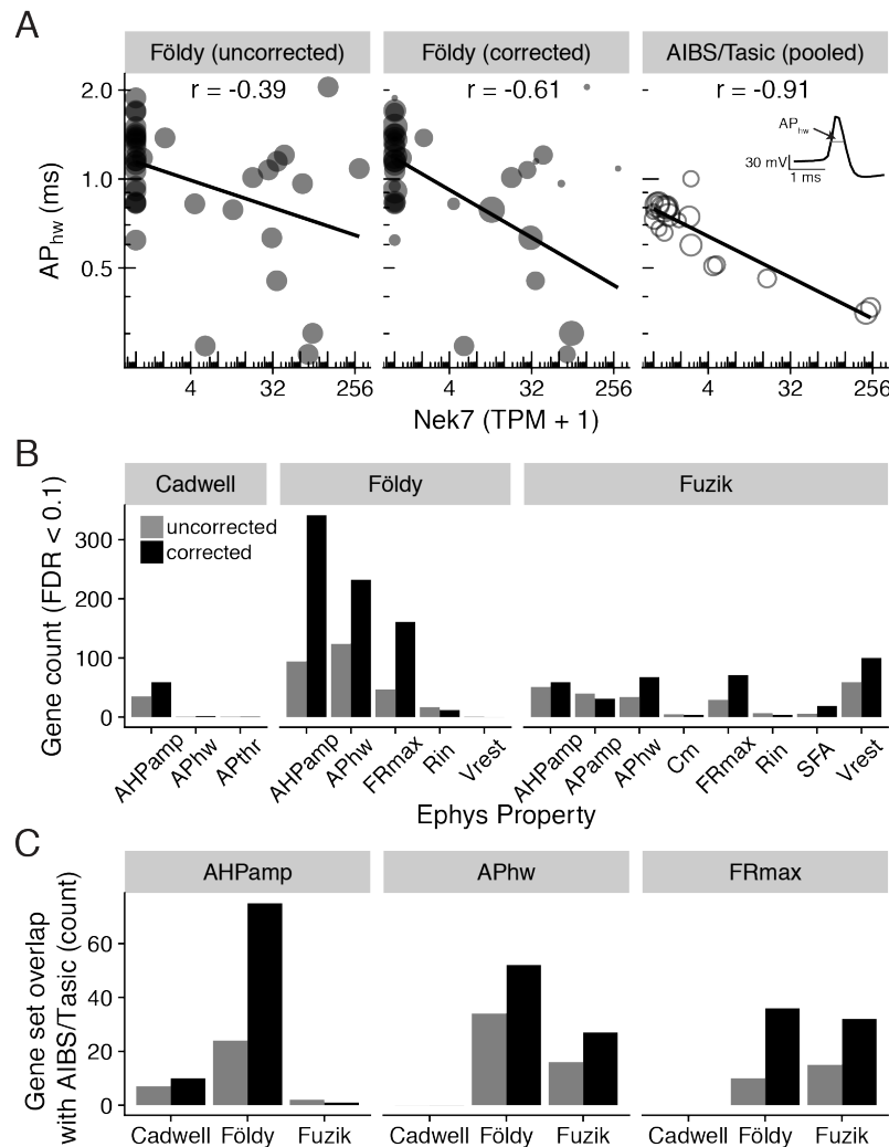
Figure 4. Adjusting for patch-seq experimental confounds improves the correspondence with electrophysiological measures. A) Comparison of gene expression (Nek7; x-axis) with electrophysiological features (action potential half-width; AP hwh ; y-axis). Left panel shows single-cell samples (circles) from the Földy dataset. Middle panel shows same data as left, but size of circles proportional to each sample's quality score, defined as the similarity of marker
