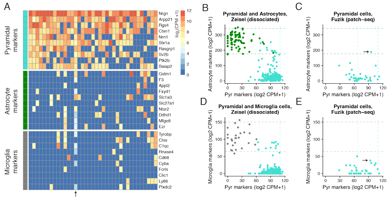
Supplement Figure 1. Expression of cell type-specific marker genes in patch-seq samples from Fuzik. A) Gene expression profiles for sampled pyramidal cells for various cell type-specific markers. B) Summed expression of cell type-specific marker genes for Pyramidal cell (x-axis) and Astrocyte (y-axis) markers. Dots reflect cortical Pyramidal cell (turquoise) and Astrocyte (green) single cells collected in the Zeisel dataset, based on dissociated scRNAseq. Dashed lines reflect 95% intervals of marker expression for each cell type. C) Same as B, but showing summed marker expression for Pyramidal cells shown in A based on patch-seq data. Arrow denotes the same single-cell highlighted in A. D,E) Same as B and C, but showing comparison of microglial marker expression.
