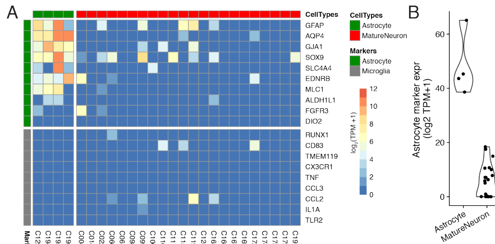
Figure 2. Expression of cell type-specific marker genes in patch-seq samples obtained from human astrocytes and neurons differentiated in culture from the Bardy dataset. A) Gene expression profiles for differentiated astrocytes (green) and electrophysiologically-mature neurons (red) for astrocyte and microglial-specific (grey) marker genes. Each column reflects a single-cell sample. Two astrocyte cells were removed because they expressed fewer than 3 astrocyte markers. B) Summed astrocyte marker expression for astrocyte and mature neuron single-cells, for the same cells shown in part A.
