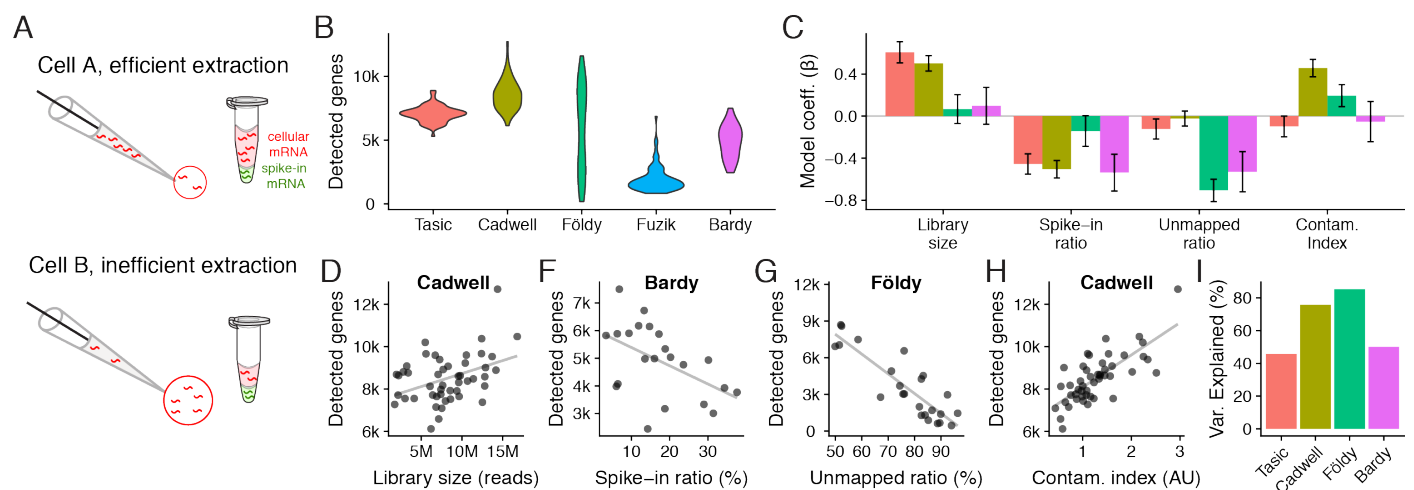
Figure 3. Patch-seq experimental confounds affect the numbers of genes detected per cell. A) Schematic illustrating how spike-in mRNAs can be used to estimate how much mRNA was extracted per cell. B) Violin plots showing numbers of protein-coding genes detected per cell across patch-seq datasets or the Ndnf subset of the Tasic dissociated-cell dataset. C) Technical factors associated with numbers of genes detected per cell across datasets (dataset color shown in B). Bars show standardized beta model coefficients with y-axis in units of standard deviations, allowing comparison of effects across factors and across datasets. Error bars indicate coefficient standard deviations. Positive (negative) coefficients indicate factor is correlated with increased (decreased) gene counts. Regression models calculated using only cells containing mRNA spike-ins. D-H) Examples of univariate relationships between technical factors and detected gene count per cell (dots) across patch-seq datasets. Grey line shows best fit line. D) Library size (count of sequenced reads per cell). F) Spike-ins as a fraction of all sequenced reads per cell. Samples with lower cellular mRNA content (indicated by higher spike-in ratios) have lower gene counts. G) Unmapped ratio, calculated as the ratio of exonic reads to all other reads (excluding spike-ins). H) Cellular contamination index, quantified by summing normalized contamination values across tested cell types (arbitrary units). I) Overall percent variance explained by each dataset-specific statistical model shown in E.
