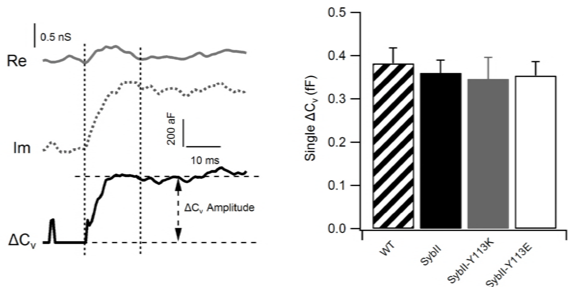
Figure 3. Single capacitance measurement by cell-attached capacitance. (A) Real part (Re, gray
