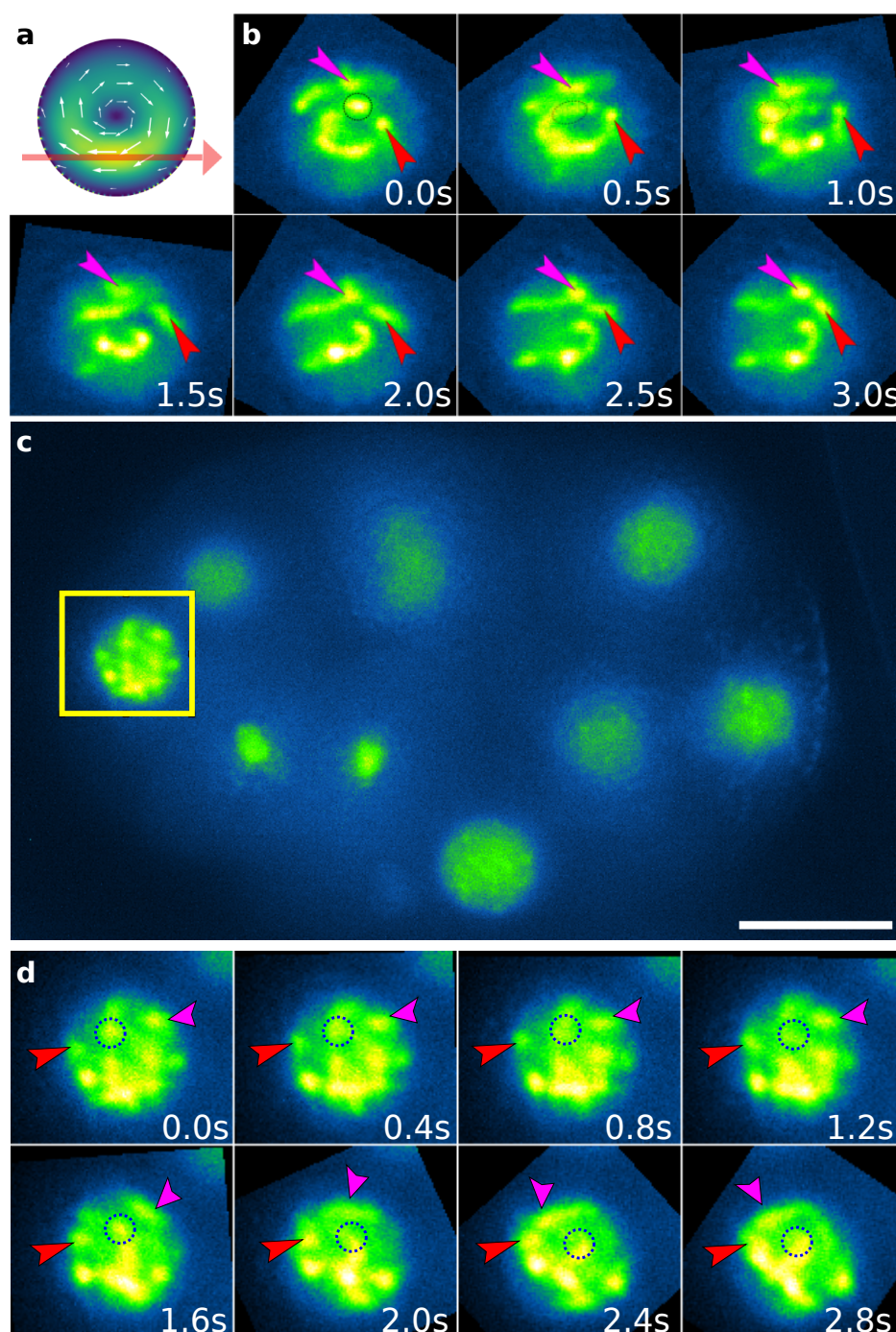
Figure 3: Prophase chromosomes are free to exchange neighbors
