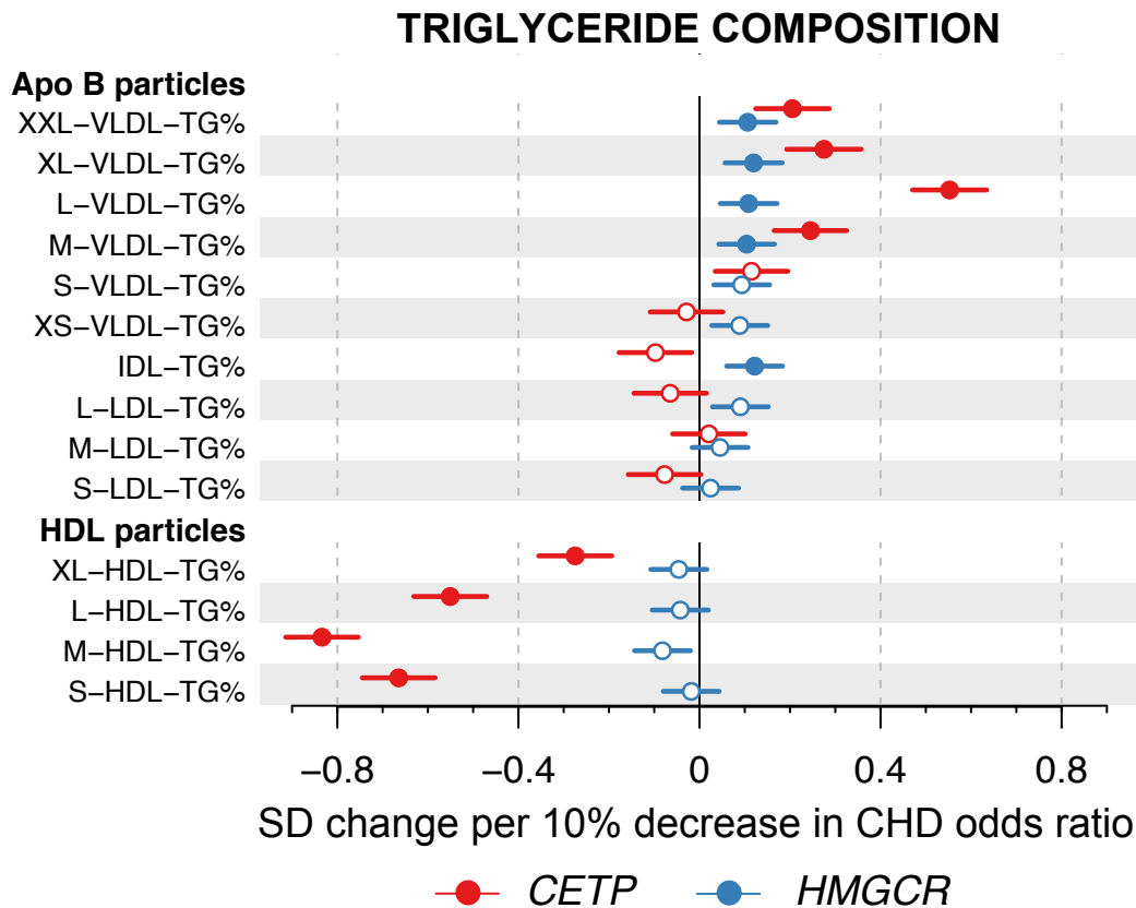
Figure 4. Associations of genetic variants in CETP rs247617 (red) and HMGCR rs12916 (blue) with the triglyceride composition of size-specific lipoprotein particles. The estimates are as defined in the caption for Fig. 1 and the lipoprotein subclasses are as defined in the captions for Fig. 1 and Fig. 3.
