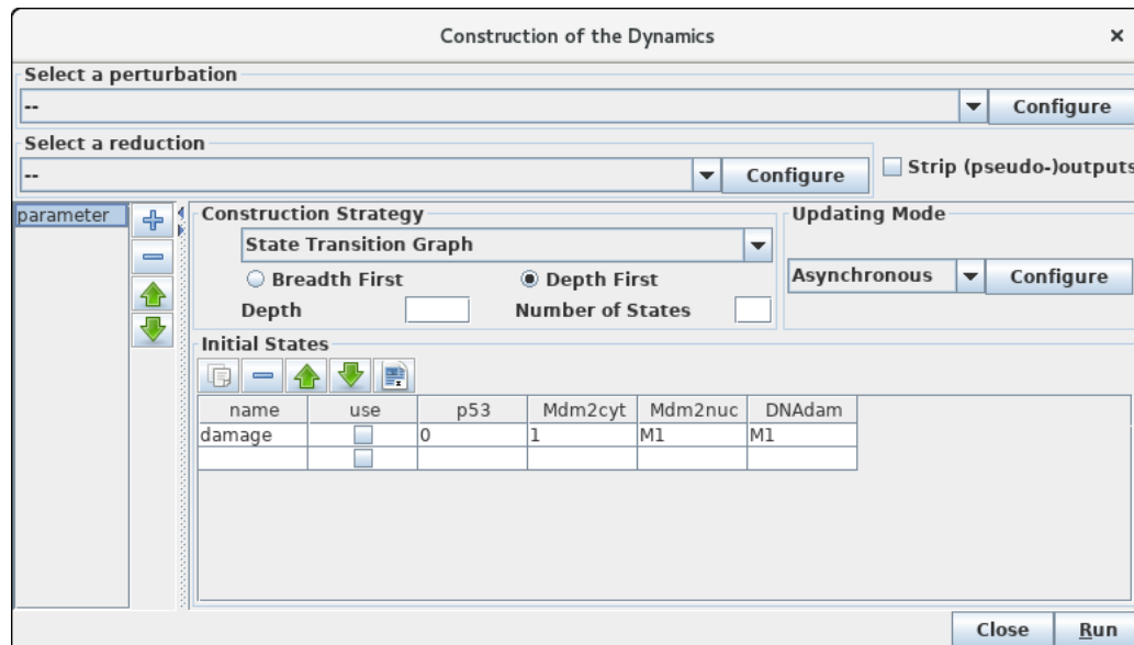
Figure 5: Launching of the construction of a state transition graph. This panel is obtained when selecting Run Simulation from the Tools scrolling menu in GINsim main window. The default simulation settings are shown, i.e. the construction of a state transition graph using the asynchronous updating, with no specified initial state (meaning that all states are considered in the simulation). Hitting the Run button will generate the corresponding state transition graph in a new window (see Figure 6). In the table under Initial States , one can define one or several initial states from which the dynamics will be constructed (just type the desired values in a row along with an optional name). Each row of the table defines a single (or a group) of states, and the check-boxes allow to select the states to be used for a simulation. The levels are specified for each node in the corresponding table cell. Nodes for which values are left free are denoted by stars (*). Initial states can be reordered, deleted and duplicated using the buttons just above the table. Here, a unique initial state has been defined, but not selected for simulation: the state 0111 ( i.e. with p53 set to 0, and the three other nodes set to 1). Note that M1 emphasises the fact that the value 1 is the maximal level for Mdm2nuc and for DNAdam. Several parameter configurations can be created and stored using the + button on the left side.
