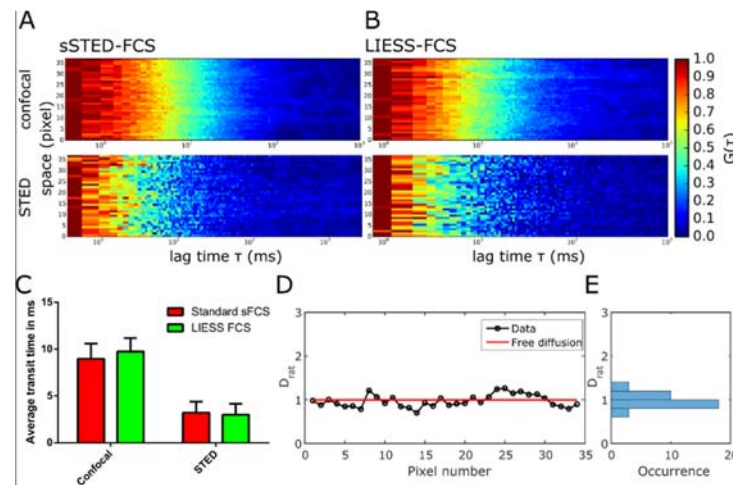
Figure 2: Experimental LIESS-FCS recordings of free diffusion in SLBs (Abberior Star Red labelled DPPE in DOPC/Cholesterol). A) Representative correlation carpets of confocal ( d_{\text{conf}} = 240 nm, upper panel) and STED ( d_{\text{STED}} = 100 nm, lower panel) from conventional sSTED-FCS and B) LIESS-FCS correlation carpets in confocal ( d_{\text{conf}} = 240 nm, upper panel) and STED ( d_{\text{STED}} = 100 nm, lower panel, measurement time 150 s, 1.36 \mu\text{m} scan). C) Values of transit times (average and standard deviation of the mean as error bars) determined from confocal and STED correlation carpets of the sSTED-FCS and LIESS-FCS recordings (72 curves in confocal and STED), indicating no significant difference between sSTED- and LIESS-FCS. D) Values of D_{\text{rat}} along the pixels of the scanned line resulting from the analysis of the LIESS-FCS correlation carpets and E) frequency histogram indicating fluctuations around D_{\text{rat}} = 1.0 i.e. free diffusion (red line in D).
