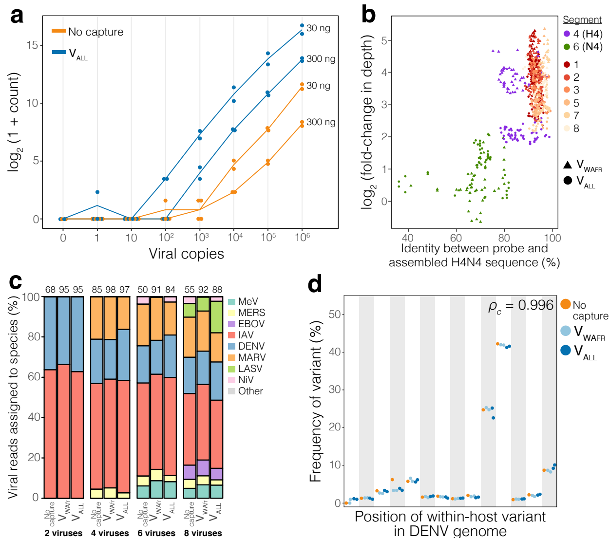
Figure 3 – Characterizing improvement in detection and detection of within-sample diversity. (a) Amount of viral material sequenced in a dilution series of viral input in two amounts of human RNA background. There are n = 2 technical replicates for each choice of input copies, background amount, and use of capture ( n = 1 replicate for the negative control with 0 copies). Each dot indicates number of reads, among 200,000 in total, sequenced from a replicate; line is through the mean of the replicates. Label to the right of each line indicates amount of background material. (b) Relation between probe-target identity and enrichment in read depth, as seen after capture with V ALL and with V WAFR on an Influenza A virus sample of subtype H4N4 (IAV-SM5). Each point represents a window in the IAV genome. Identity between the probe and assembled H4N4 sequence is a measure of identity between the sequence in that window and the top 25% of probe sequences that map to it (see Methods for details). Fold-change in depth is averaged over the window. No sequences of segment 6 (N) of the N4 subtypes were included in the design of V ALL or V WAFR . (c) Effect of capture on estimated frequency of within-sample co-infections. RNA of 2, 4, 6, and 8 viral species were spiked into extracted RNA from healthy human plasma and then captured with V ALL and V WAFR . Values on top are the percent of all sequenced reads that are viral. We did not detect Nipah virus (NiV) using the V WAFR probe set because this virus was not present in that design. (d) Effect of capture on estimated frequency of within-host variants, shown in positions across three dengue virus samples: DENV-SM1, DENV-SM2, and DENV-SM5. Capture with V ALL and V WAFR was each performed on n = 2 replicates of the same library. \rho_c indicates concordance correlation coefficient between pre- and post-capture frequencies.
