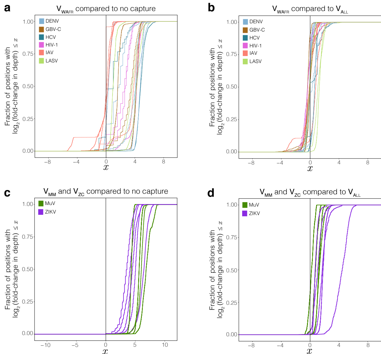
Supplementary Figure 8 – Enrichment in read depth with focused probe sets. (a) Distribution of the enrichment in read depth, across viral genomes, provided by capture with V_{WAFR} . Each curve represents a viral genome. At each position across a genome, the post-capture read depth is divided by the pre-capture depth, and the plotted curve is the empirical cumulative distribution of the log of these fold-change values. (b) Distribution of the enrichment in read depth, across viral genomes, provided by V_{WAFR} over V_{ALL} . At each position across a genome, the read depth following capture with V_{WAFR} is divided by the depth following capture with V_{ALL} , and the plotted curve is the empirical cumulative distribution of the log of these fold-change values. (c) Same as (a), but for the two-virus probe sets V_{MM} and V_{ZC} . The mumps curves (green) show enrichment provided by V_{MM} against pre-capture, and the Zika curves (purple) show enrichment provided by V_{ZC} against pre-capture. (d) Same as (b), but for the two-virus probe sets V_{MM} and V_{ZC} . The mumps curves (green) show enrichment provided by V_{MM} against V_{ALL} , and the Zika curves (purple) show enrichment provided by V_{ZC} against V_{ALL} .
