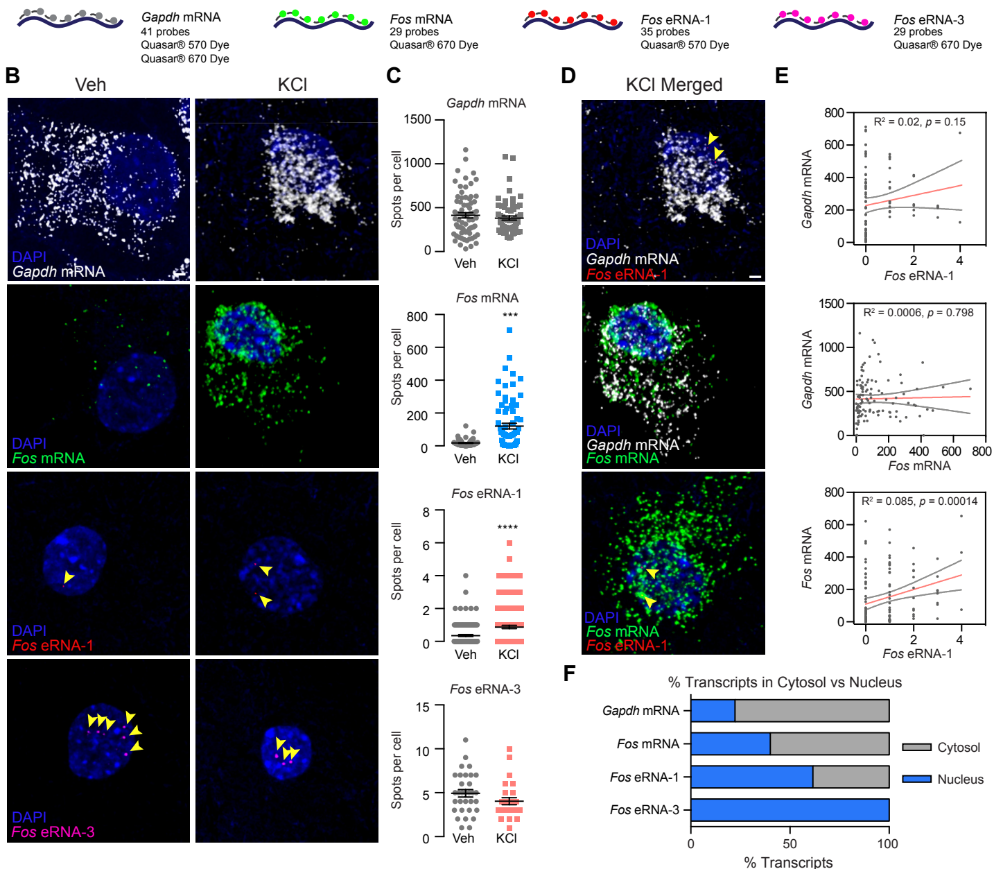
Figure 4. Cellular localization of Fos eRNA and mRNA. A , Illustration of smFISH probe sets indicating number of probes, dye, and LUT. B , smFISH for Gapdh mRNA (Quasar® 570), Fos mRNA (Quasar® 670), eRNA-1 (Quasar® 570) and eRNA-3 (Quasar® 670) transcripts at baseline and after KCl-mediated depolarization. Cell nuclei are stained with DAPI (blue), RNA transcripts are marked by smFISH probes (gray, green, red, and pink). Scale bar 2 \mu m. C , Quantification of spot detection using StarSearch. Number of detected spots for Fos mRNA and Fos eRNA-1 changes significantly after stimulation (Mann-Whitney test for Gapdh n(veh)=72, n(KCl)=63, U=2187, p>0.05; Fos mRNA n(veh)=77, n(KCl)=76, U=1929, p<0.001; eRNA-1 n(veh)=124, n(KCl)=141, U=6540, p>0.0001; eRNA-3 n(veh)=32, n(KCl)=27, U=316.5, p>0.05). D , Merged KCl images of Gapdh mRNA, Fos mRNA and eRNA-1. E , Comparison and correlation of detected Gapdh mRNA, Fos mRNA and eRNA-1 spots per cell. There is a significant correlation between Fos mRNA (Quasar® 670) and Fos eRNA-1 (Quasar® 570) (Pearson r, R-square=0.08481, p=0.0014) but not between Gapdh mRNA (Quasar® 570) and Fos mRNA (Quasar® 670) or Gapdh mRNA (Quasar® 570) and eRNA-1 (Quasar® 570) (Pearson r for Gapdh mRNA and Fos mRNA R-square=0.000586, p=0.7982; Gapdh mRNA and eRNA-1 R-square=0.02344, p=0.1451). F , Quantification of smFISH for Gapdh mRNA, Fos mRNA, Fos eRNA-1 and Fos eRNA-3 transcripts in the cytosol vs nucleus. Data expressed as mean \pm s.e.m. Multiple comparisons, *p<0.05, **p<0.01, ***p<0.001, ****p<0.0001.
