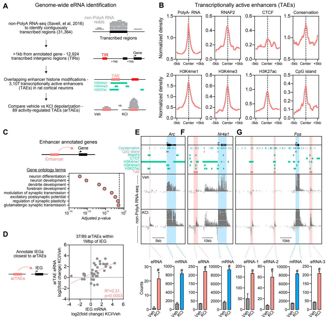
Figure 1. Genome-wide characterization of eRNAs. A , Analysis pipeline for localization and quantification of transcriptionally active enhancers (TAEs), and genome-wide comparisons of eRNA expression following neuronal depolarization. Non-PolyA RNA-seq datasets from previous publication using cultured rat cortical neurons (Savell, et al., 2016) were used to identify contiguously transcribed regions, which were filtered to remove transcribed regions overlapping annotated genes. Of 12,924 transcribed intergenic regions (TIRs), 24% (3,107 loci) overlapped histone modifications consistent with active or poised enhancers, and were designated TAEs. Of these, 89 met genome-wide criteria for differential expression following 1hr neuronal depolarization with 25 mM potassium chloride (KCl), and were designated activity-regulated TAEs (arTAEs). B , Transcriptionally active enhancers exhibit elevated RNAP2 occupancy, CTCF binding, sequence conservation (phastCons13way score), histone modifications (H3K4me1, H3K4me3, H3K27ac), and CpG island density as compared to surrounding regions. Chromatin immunoprecipitation datasets were obtained from the adult mouse cortex (ENCODE project) and lifted over to the rat Rn5 genome assembly. C , Gene ontology for 1,362 unique genes closest to TAEs. TAEs are enriched near genes that regulate neuronal function and synaptic transmission. D , eRNA-mRNA pairs were determined by annotation of closest immediate early genes (IEGs) induced by neuronal depolarization with 25 mM KCl, with a 1Mbp distance cutoff. Correlation between differential expression of IEG mRNAs following KCl depolarization and differential expression of eRNA from closest arTAEs following depolarization. Values are expressed as \log_2(\text{fold change}) of eRNA or mRNA counts used for comparison in DESeq2. Correlation determined with linear regression. E-G , Top, Genome browser tracks showing Non-PolyA RNA expression at three KCl-regulated IEGs ( Arc , Nr4a1 , and Fos ), relative to tracks marking conserved DNA elements, CpG islands, RNAP2 and CTCF binding, and enhancer-linked histone modifications. Our pipeline identified one or more TAEs near each IEG. Bottom, RNA-seq count quantification of transcripts from TAEs (eRNAs in pink, from non-PolyA libraries), and mRNAs (in blue, from separate PolyA+ libraries). *FDR < 0.05 for DESeq2 comparison of differential expression between vehicle and KCl groups.
