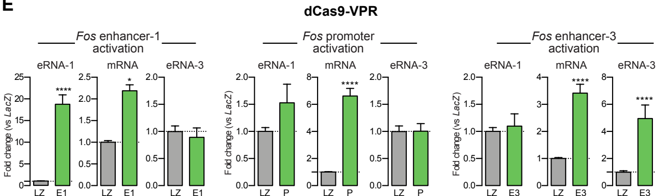
Supplementary Figure 2. Enhancer activation increases Fos eRNA and mRNA expression. A , C6 cells 16h post nucleofection with VP64 containing plasmids (dCas9-VP64 expression marked by GFP reporter, gRNA expression marked by mCherry reporter). B , Illustration of CRISPR activation (CRISPRa) strategy for site-specific targeting of the transcriptional activator VP64. C , Target sites of gRNAs at 3 Fos enhancers, and one Fos promoter site. D , RT-qPCR analysis of VP64 mediated induction of Fos eRNAs and mRNA when targeted to individual sites surrounding the Fos gene, compared to the non-targeting lacZ control. CRISPRa resulted in site-specific upregulation of selected eRNAs and mRNA. Increasing Fos eRNA-1 and eRNA-3 levels resulted in increased Fos mRNA levels but not vice versa (n=9 per group; one-way ANOVA for eRNA-1 (F(4,40)=66.22, p<0.0001), eRNA-2 (F(4,40)=22.85, p<0.0001), eRNA-3 (F(4,40)=10.55, p<0.0001), and mRNA (F(4,40)=14.66, p<0.0001); Dunnett's multiple comparisons test). E , RT-qPCR analysis of VPR mediated induction of Fos eRNAs and mRNA when targeted to individual sites. CRISPRa resulted in site specific up-regulation of selected eRNAs and mRNA compared to non-targeting lacZ control (n=9 per group; one-way ANOVA for eRNA-1 (F(4,40)=49.47, p<0.0001), eRNA-2 (F(4,40)=12.58, p<0.0001), eRNA-3 (F(4,40)=18.52, p<0.0001), and mRNA (F(4,40)=46.43, p<0.0001); Dunnett's multiple comparisons test. Increasing Fos eRNA1 and eRNA-3 levels resulted in increased mRNA levels but not vice versa. Data expressed as mean \pm s.e.m. Multiple comparisons, *p<0.05, **p<0.01, ***p<0.001, ****p<0.0001.
