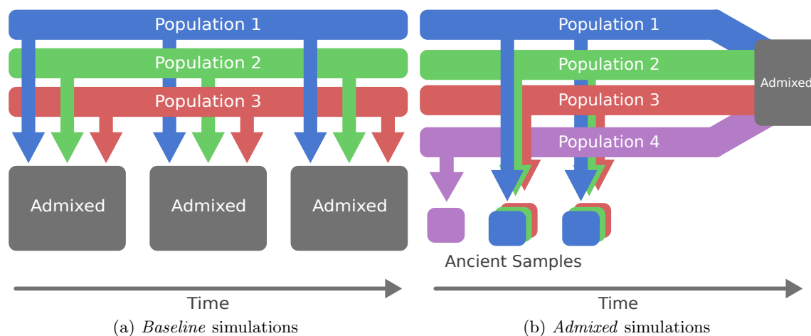
Fig. 2. Simulation scenarios explored with Dystrust. (a) Baseline simulation scenario. Three populations were simulated that admixed at three time points. Individuals were sampled from the admixed populations. (b) Admixed simulation scenario. Ancient individuals were sampled from four unadmixed populations that merged to form a modern admixed population. Modern samples were from the admixed population.
