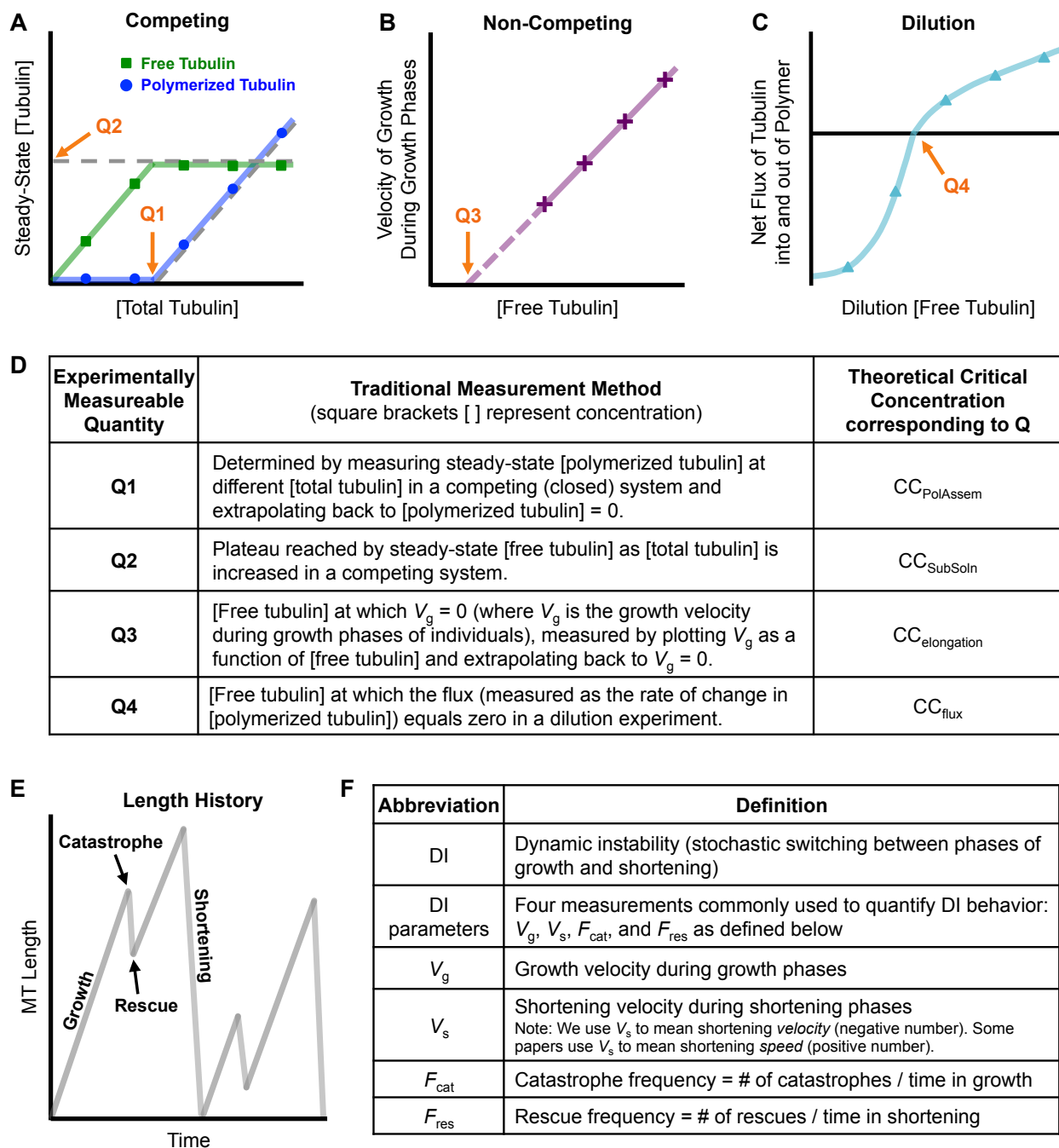
Figure 1: Classical understanding of microtubule (MT) polymer assembly behavior. See Table 1 for additional description of the critical concentration measurements depicted here. [Free tubulin] is the concentration of tubulin dimers in solution, [polymerized tubulin] is the concentration of tubulin dimers in polymerized form, and [total tubulin] = [free tubulin] + [polymerized tubulin]. (A) In a competing (closed) system, [total tubulin] is held constant over time and MTs compete for tubulin. As typically presented in textbooks, the critical concentration (CC) can be
