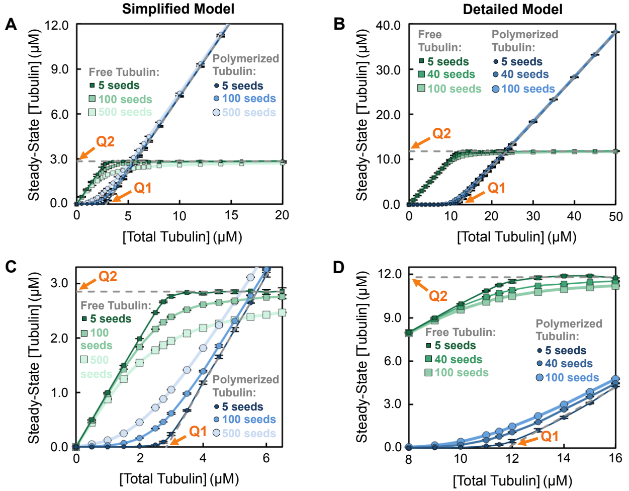
Figure 4: Impact of changing the number of microtubule seeds. Steady-state concentrations of free (squares) and polymerized (circles) tubulin in a competing system as in Figure 3A-B . ( A,C ) Simplified model with MTs growing from 5, 100, or 500 stable MT seeds (data for 100 seeds re-plotted from Figure 3A ). ( B,D ) Detailed model with MTs growing from 5, 40, or 100 stable MT seeds (data for 40 seeds re-plotted from Figure 3B ). Panels 4C-D show zoom-ins of the data plotted in panels 4A-B , respectively. The darker curves with smaller symbols correspond to fewer seeds and the lighter curves with larger symbols correspond to more seeds. Interpretation: These data show that changing the number of stable MT seeds alters the approach to the asymptotes determining Q1 and Q2 (dashed grey lines re-plotted here from Figure 3A-B ), but does not change the value of Q1 \approx Q2 . Methods: Data points represent the mean \pm one standard deviation of the values obtained in three independent runs of the simulations. Similar to Figure 3 , [free tubulin] and [polymerized tubulin] from each run were averaged over a period of time after polymer-mass steady state was reached. The time to reach this steady state depends on the number of stable MT seeds (see Figure S2 ). For the simplified model, the averages of [free tubulin] and [polymerized tubulin] were taken from 120 to 150 minutes for 5 MT seeds and from 15 to 30 minutes for 100 and 500 MT seeds. For the detailed model, the averages were taken from 100 to 150 minutes for 5 MT seeds and from 30 to 60 minutes for 40 and 100 MT seeds. We were able to use a higher number of seeds in the simplified model than in the detailed model because it is more computationally efficient.
