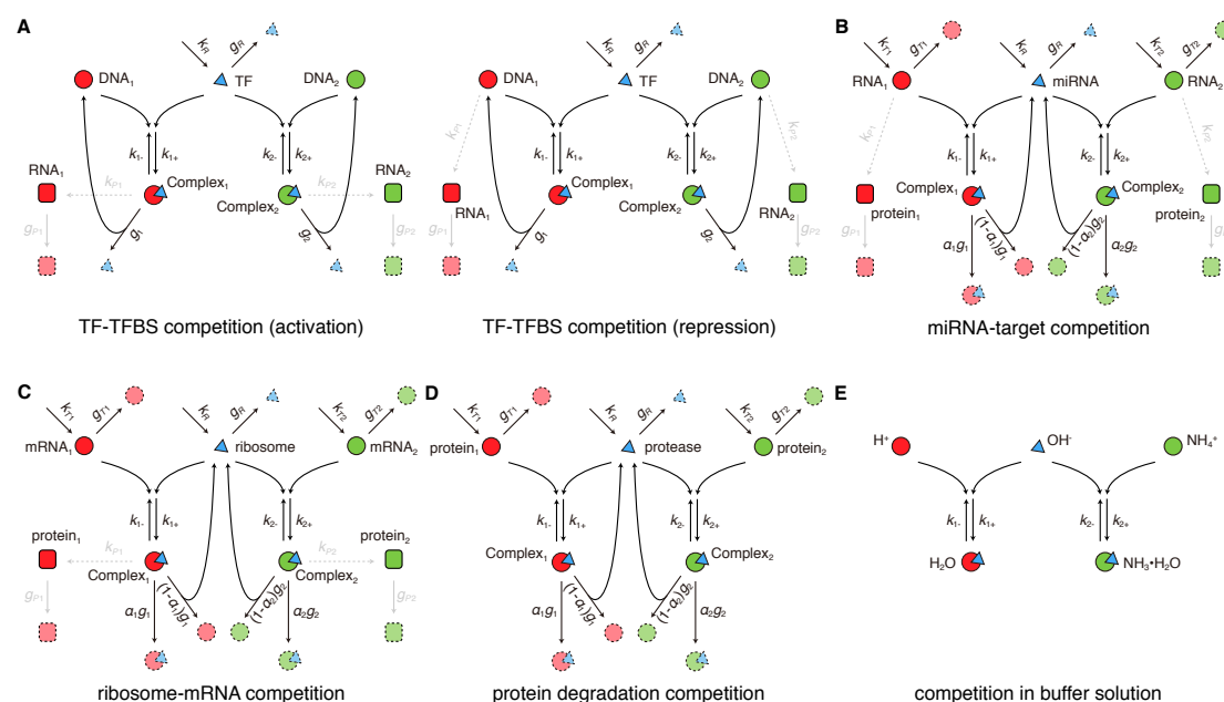
Figure S1 Detailed descriptions under the unified coarse-grained competition motif model for diverse competition scenarios.
